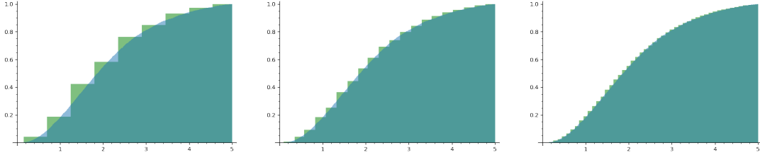
Figure 6: Case e = 7 . Convergence to \sum_{k=1}^3 \Gamma(1, \sin \frac{k\pi}{7}) .
