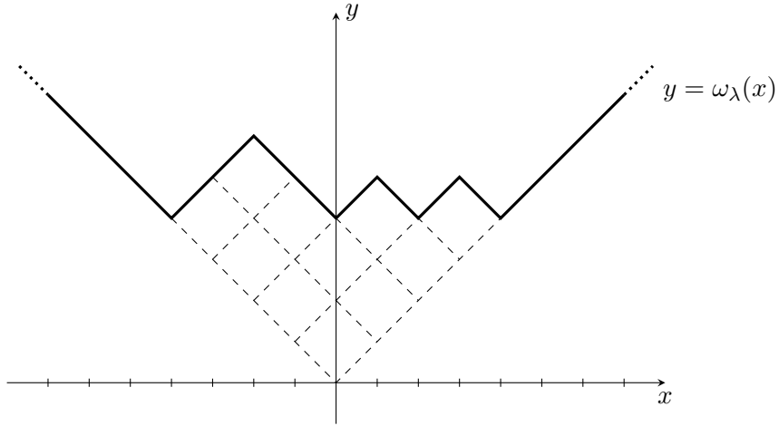
Figure 2: Russian convention for the Young diagram of \lambda = (4, 3, 2, 2)
