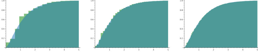
Figure 5: Case e = 4 . Convergence to \Gamma(1, \frac{1}{\sqrt{2}}) + \Gamma(\frac{1}{2}, 1) .
