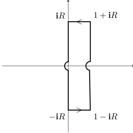
Figure 4: Contour C_R
