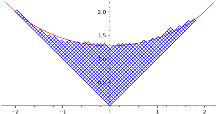
Figure 1: Universal limit shape for the partitions under the Plancherel measure (here with n = 700 ).
