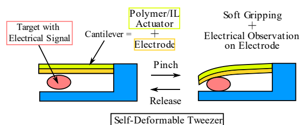
Figure 1. Self-deformable tweezer enables mechanical gripping and electrical observation simultaneously.
