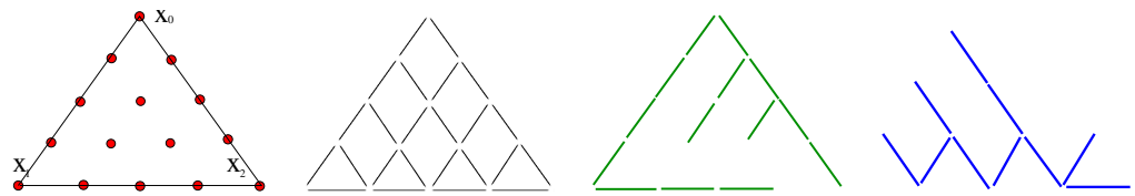
Figure 1. For r + 1 = 4 , in a mesh triangle t = [x_0, x_1, x_2] , from left to right, are drawn, respectively, the small nodes of the principal lattice, the active small edges of the graph \mathcal{G} associated with the small-edge-to-small-node incidence matrix G , a spanning tree in \mathcal{G} and its cotree.
