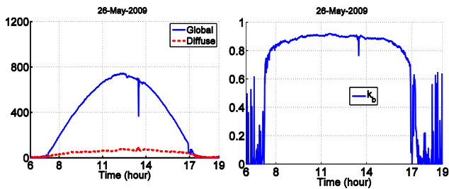
Figure 5 Clear sky day solar radiation on the left [ \text{W/m}^2 ], and the k_b index on the right
