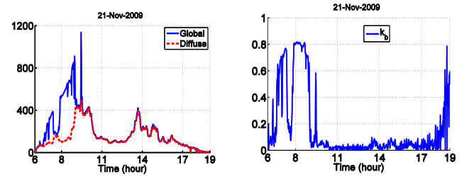
Figure 6 Intermittent cloudy day solar radiation on the left [ \text{W/m}^2 ], and the k_b index on the right
