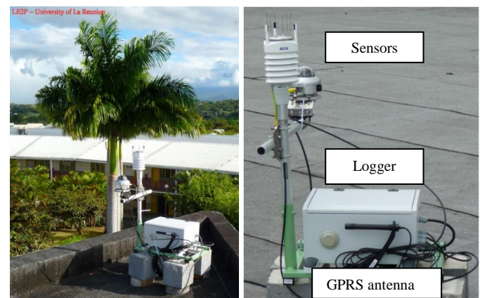
Figure 4 An RCI_GS station with SPN1 sensor, Vaisala meteorological suite, logger and communications hardware
