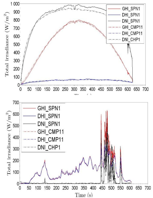
Figure 2 Comparison of GHI, DHI and DNI from the SPN1 sensor (solid) and collocated reference instruments (dotted) for a clear sky day (top) and a partial cloudy day (bottom)
