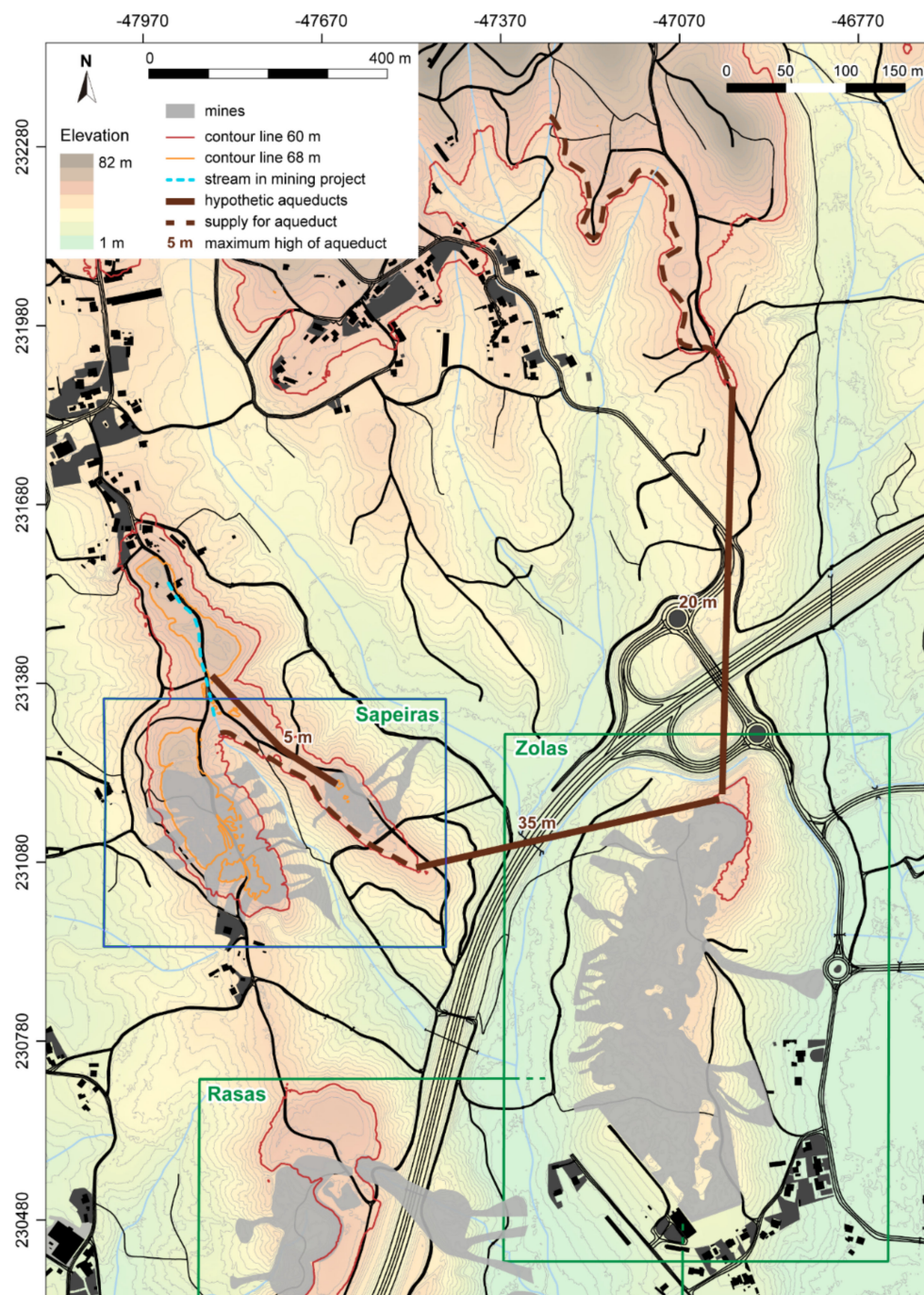
Figure 20. General view of the relief around Sapeiras and Zolas mine, overlapped with 1:10,000 vector cartography of the Viana do Castelo Municipality.
