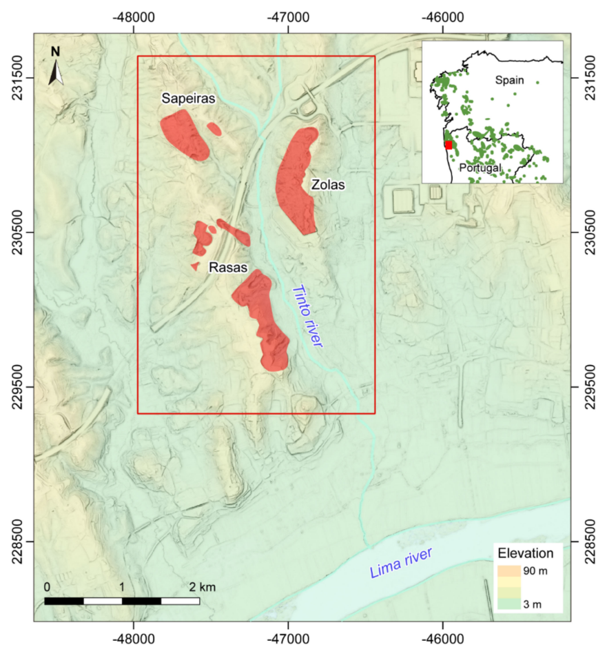
Figure 1. Location of the study area. Mining areas are highlighted in red overlaying light detection and ranging (LiDAR) elevation data. The Northwest Iberia map (right upper corner) gives the location of the study area in relation to tin deposits (green dots) after [2].
