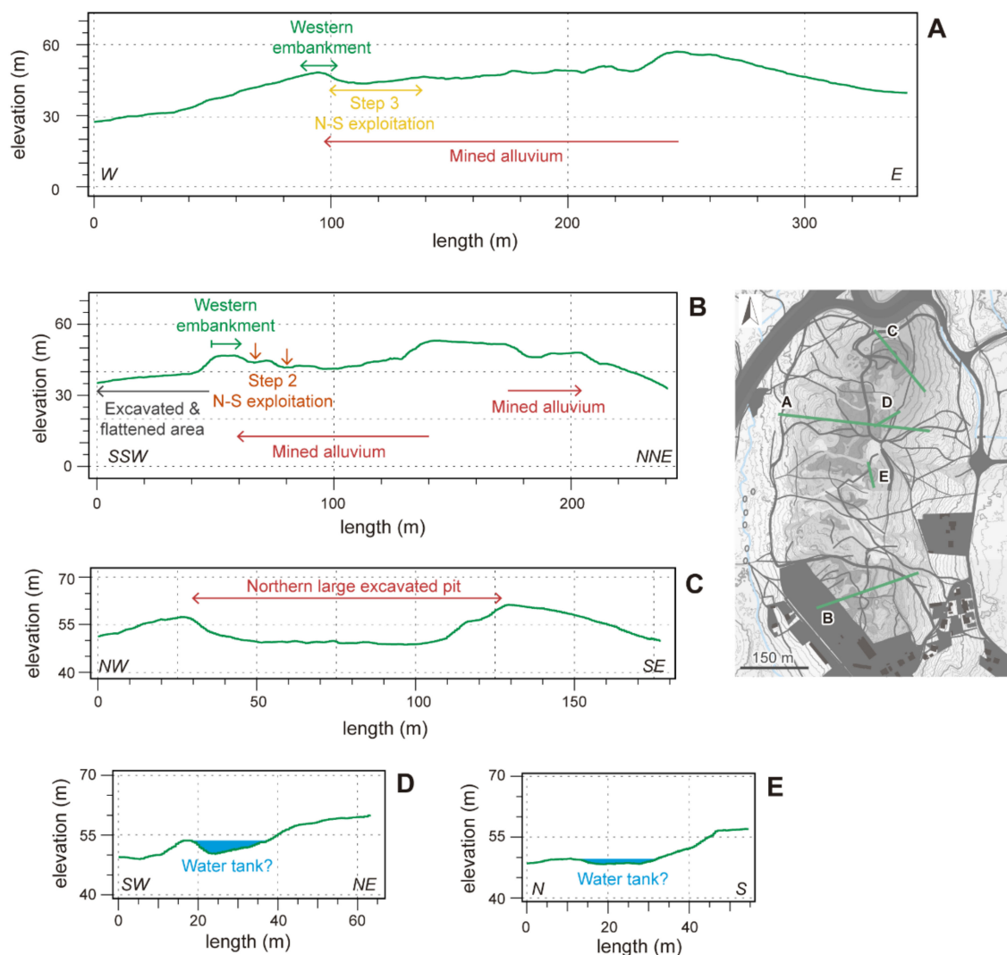
Figure 16. (A–E) sections of Zolas mine.
