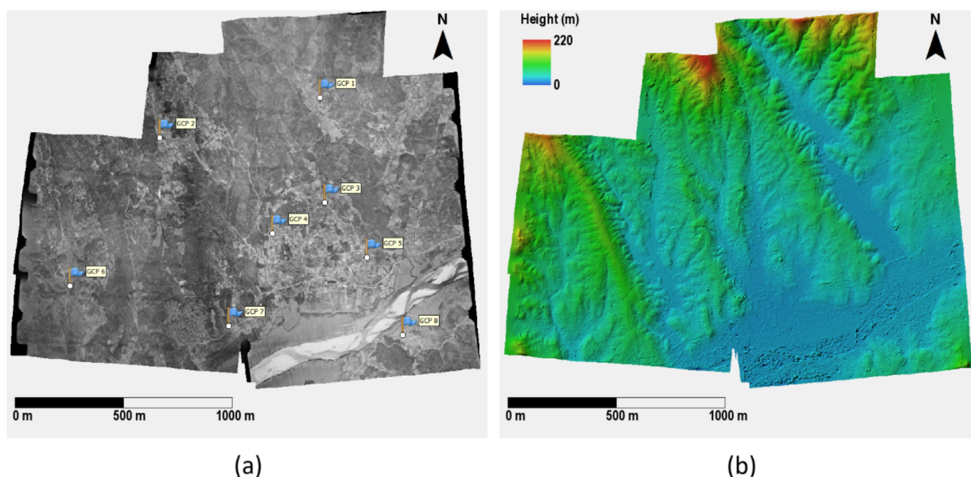
Figure 4. Results of processing the SPLAL dataset: (a) Orthomosaic built with 10 photos, with the eight ground control points (GCPs) used; (b) digital surface model (DSM) generated, with heights coded in colours and with shaded relief.
