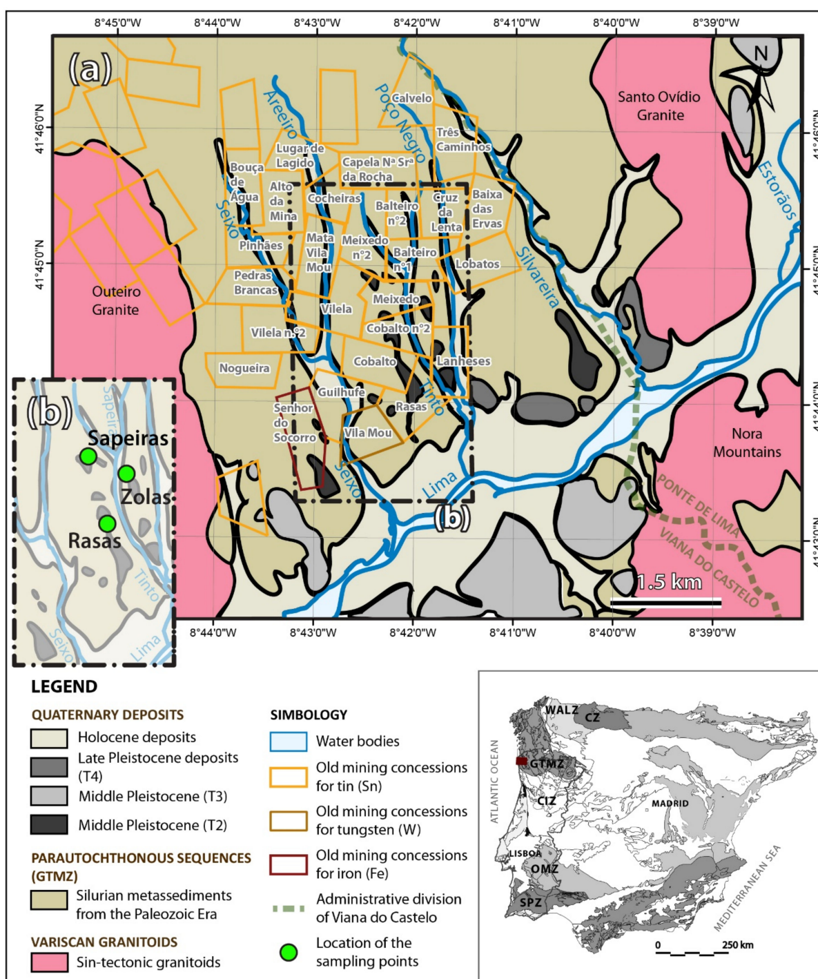
Figure 8. Geological map of the Lima river catchment basin with its Cenozoic sedimentation (adapted from [42]) with (a) the mining concessions of the 20th-century [19] in the municipality of Viana do Castelo (depicted as old mining concessions) and (b) location of the sampling points for Sapeiras, Zolas and Rasas which are over T2 old terraces [43].
