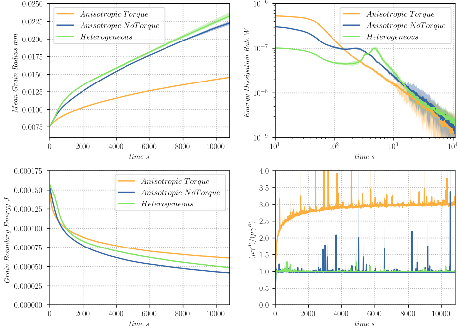
Figure 5: Evolution of different averaged or integrated quantities as a function of time, (top-left) arithmetic mean grain radius \bar{r} , (top-right) energy dissipation rate ( dE/dt versus t ), (bottom-left) total grain boundary energy and (bottom-right) ratio between the mean apparent reduced mobility and the real one (see Eq.6). Results for each case are averaged from the results of the four different initial tessellations, with the range of results indicated by semi-transparent shading of the same color as the corresponding curve. (Wherever this shading is not visible, the maximum and minimum values are nearly identical with the average.)
