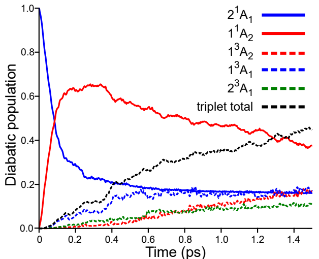
FIG. 3. Evolution of diabatic populations for the singlets 2^1A_1 ( 1\pi\pi^* , solid blue) and 1^1A_2 ( 1n\pi^* , solid red), and triplets 1^3A_2 ( 3n\pi^* , dashed red), 1^3A_1 ( 3\pi\pi^* , dashed blue) and 2^3A_1 (dashed green). The black dashed line corresponds to the sum of all triplet population. The dynamics have been started from the 2^1A_1 state.
