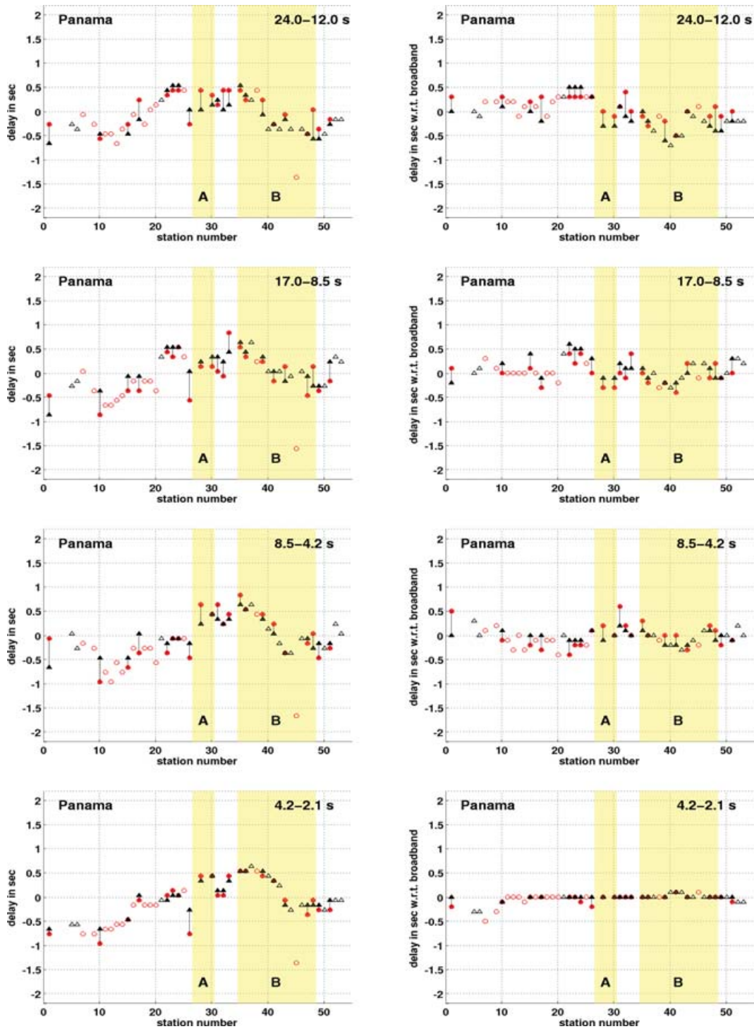
Figure 12. Panama quplet: finite frequency traveltimes (left column) and traveltimes dispersion (right column), along RISTRA. Measurements from the two events generally agree very well. Region A: the negative dispersion anomaly around stations 28–30 is visible; no data for station 29. Region B: clear and broad negative dispersion anomaly centred on station 41, gradually dies away towards high frequencies. (Note that in this example, dispersion plots directly compare frequency bands since broad-band traveltimes are indistinguishable from those at the highest frequencies.)
