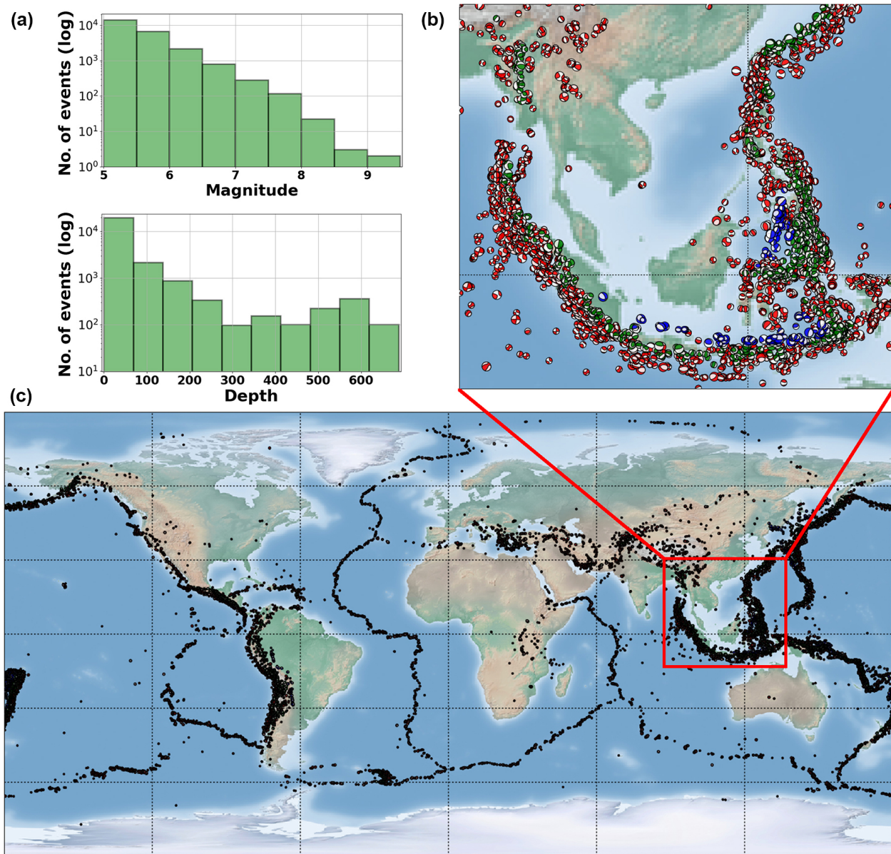
Figure 2. obsypyDMT --datapath neic_event_dir --min_date 1990-01-01 --max_date 2017-01-01 --min_mag 5.0 --event_catalog NEIC_USGS --event_info --plot_seismicity Global seismicity map of archived earthquakes in NEIC catalog of a magnitude of more than 5.0 that occurred between 1990 and 2016. One command queried the NEIC catalog, stored and organized the retrieved information and generated the seismicity map. (No actual waveform data were queried in this example.) The results of some basic statistics (magnitude and depth histograms) are also generated and plotted automatically (a). Note the rendering of colored beach balls in the map inset (deepest seismicity in the foreground). The global map also contains beach balls rather than just simple black dots, but they do not become apparent at this zoom level.
