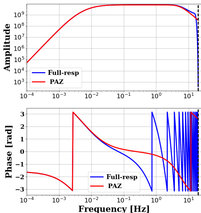
Figure 7. obspyDMT --plot_stationxml --plotxml_paz --plotxml_min_freq 0.0001 --datapath /path/to/STXML.GT.LBTB.00.BHZ Transfer function spectra (amplitude and phase) of a Geotech KS-54000 borehole seismometer (GT.LBTB) in Botswana. Blue lines show transfer function components computed for all filter stages in the StationXML file; red lines are for the analog part. A large discrepancy exists between the phase spectra of the two transfer functions. The deviation emerges at frequencies around 10^{-2} Hz and increases up to the Nyquist frequency. Fig. 8 shows that this difference is caused by one of the digital stages in the instrument response.
