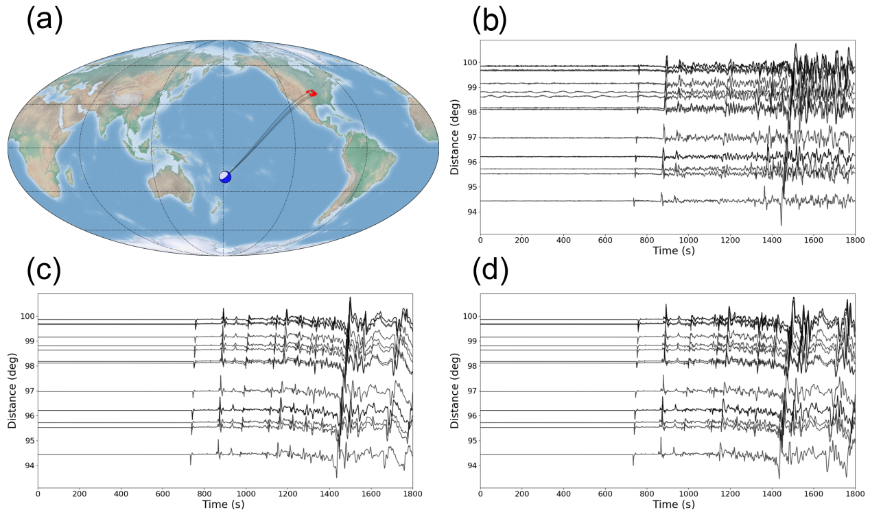
Figure 5. Observed versus modeled broadband seismograms for an earthquake of a magnitude of 6.9 M_w in the Fiji Islands region (21 July 2014, 14:54:41, at 19.802° S, 178.4° W; 615 km depth). (a) Source and receiver distribution plotted by obsipyDMT --datapath data_fiji_island --local --plot_ev --plot_focal --plot_sta --plot_ray . Note the distribution of stations with respect to the event. The options flags --min_azi , --max_azi , --min_epi and --max_epi specified minimum azimuth, maximum azimuth, minimum distance and maximum distance for station search, respectively. (b) Observed broadband waveforms plotted by obsipyDMT --datapath data_fiji_island --local --plot_waveform --plot_dir processed . (c) Synthetic seismograms retrieved from the Syngine web service for the PREM anisotropic background model. The stored waveforms are plotted by obsipyDMT --datapath data_fiji_island --local --plot_waveform --plot_dir syngine_prem_a_2s . Panel (d) is similar to (c) except for the IASP91 background model. Plotted by obsipyDMT --datapath data_fiji_island --local --plot_waveform --plot_dir syngine_iasp91_2s .
