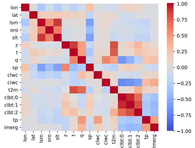
Figure 3: Spearman’s correlation of RainBench variables from April 2016 to December 2019 in latitude band [-60^\circ, 60^\circ] at pressure levels 300 hPa (about 10 km) (upper triangle) and 850 hPa (1.5 km) (lower triangle). Legend: lon : longitude, lat : latitude, lsm : land-sea mask, oro : orography (topographic relief of mountains), slt : soil type, z : geopotential height, t : temperature, q : specific humidity, sp : surface pressure, clwc : cloud liquid water content, ciwc : cloud ice water content, t2m : temperature at 2m, clbt : i i th SimSat channel, tp : ERA5 total precipitation, imerg : IMERG precipitation. All correlations in this plot are statistically significant ( p < 0.05 ).
