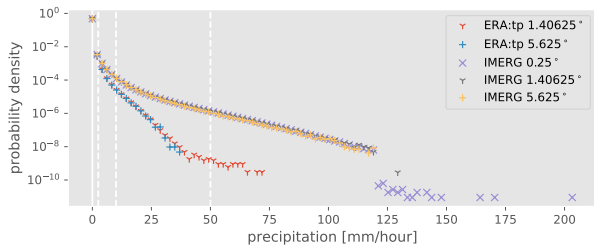
Figure 1: Precipitation histogram from 2000-2017 with ERA5 and IMERG at different resolutions. Vertical lines delineate convection rainfall types: slight ( 0\text{--}2\text{ mm h}^{-1} ), moderate ( 2\text{--}10\text{ mm h}^{-1} ), heavy ( 10\text{--}50\text{ mm h}^{-1} ), and violent (over 50\text{ mm h}^{-1} ) (MetOffice 2012).
