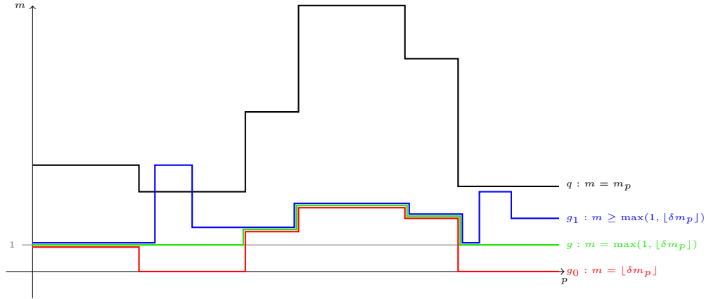
FIGURE 1 – Valuations des éléments g_0, g_1, g .
