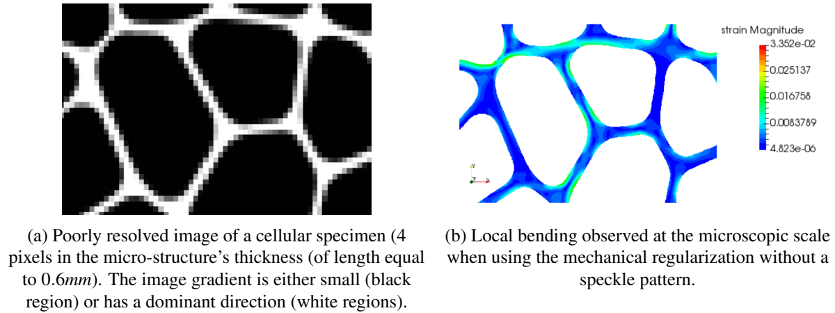
Figure 1: Strain measurement at the microscopic scale for a cellular specimen.
