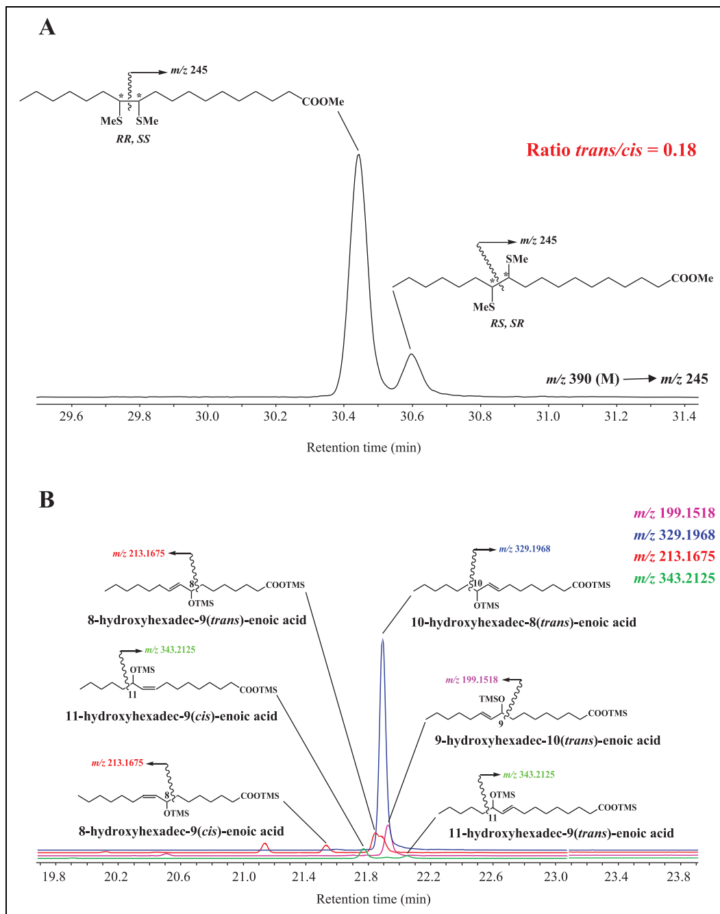
Figure 6. Lipid markers of fatty acid cis-trans isomerase and 10S-DOX-like lipoxygenase activity. (A) Multiple reaction monitoring chromatogram ( m/z 390 → 245) of DMDS adducts showing an example of cis-vaccenic isomerization ( trans/cis ratio of 0.18) in the 7–10 cm layer of sea ice collected May 8, 2005, and (B) time of flight ion chromatograms (at m/z 199.1518, 213.1675, 329.1968, and 343.2125) showing an example of the predominance of 10- trans isomer (blue line) in palmitoleic oxidation profiles of the bottommost centimeter of sea ice collected June 2, 2015, at the sampling location in Baffin Bay (Figure 1). DOI: https://doi.org/10.1525/elementa.2021.040.f6
