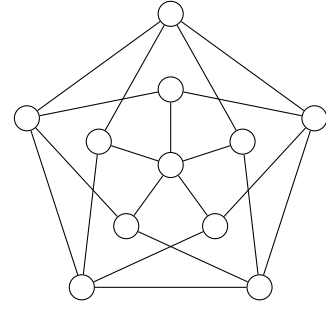
Figure 1. The Grötzsch graph
