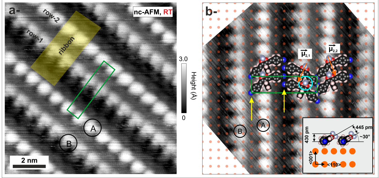
FIG. 10. (Color online). Supramolecular phase of Curc-di(CN) molecules on bulk \text{KCl}(001) , imaged by nc-AFM at room temperature. a- Nc-AFM high resolution image showing three adjacent molecular ribbons ( 10 \text{ nm} \times 10 \text{ nm} , \gamma \simeq -1.1 \cdot 10^{-2} \text{ nN} \cdot \sqrt{\text{nm}} ). Rows 1 and 2 are indicated and the 8 \times 2 supercell is overlaid as well. Type-A and B features depict two types of molecular contrast tracing two different kinds of molecule-substrate interaction and/or orientation of the molecules. These ribbons have similar features as their counterparts observed by STM on 2 \text{ ML-KCl/Au}(111) . b- Similar illustrative sketch as in fig.8. The molecular phase derived with the isomer 2 is superimposed on the image shown in a-. The experimental image has been tilted to have the \langle 010 \rangle_{\text{KCl}} axis vertical for readability. The dots depict the \text{K}^+ sites acting as anchoring points for the -\text{CN} groups of the molecules (yellow arrows). For that configuration to be possible, a vertical tilt of the molecules is mandatory (lower inset), which allows for both the compaction of the structure (hence the 8 \times 2 supercell) and the development of favorable -\text{BF}_2\text{-Ph} intermolecular interactions (cyan circle). Here, the vertical tilt angle is also 30^\circ . The model also accounts for types-A and B features.
