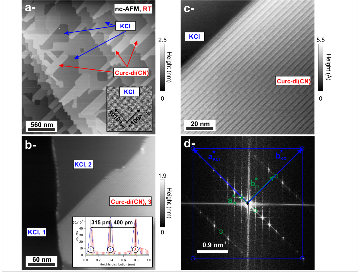
FIG. 9. (Color online). Curc-di(CN) assemblies on bulk \text{KCl}(001) , imaged by nc-AFM at room temperature. a - Large scale image of Curc-di(CN) ( \simeq 1/5 ML) showing the growth of ordered molecular domains between step edges and along the \langle 100 \rangle_{\text{KCl}} direction (cf. atomically-resolved image in inset) ( 2.8 \mu\text{m} \times 2.8 \mu\text{m} , \gamma \simeq -5.7 \cdot 10^{-3} \text{ nN} \cdot \sqrt{\text{nm}} ). b - Zoom on a molecular domain lying on a terrace from a step edge. The histogram in inset gives an estimate of the domain apparent height \simeq 400 \text{ pm} ( 300 \text{ nm} \times 300 \text{ nm} , \gamma \simeq -6.8 \cdot 10^{-3} \text{ nN} \cdot \sqrt{\text{nm}} ). c - Zoom on the molecular domain exhibiting molecular rows whose internal structure gets discernable ( 100 \text{ nm} \times 100 \text{ nm} , \gamma \simeq -8.5 \cdot 10^{-3} \text{ nN} \cdot \sqrt{\text{nm}} ). d - Fast Fourier Transform image (modulus) of image c -. The \text{KCl} unit cell ( \mathbf{a}_{\text{KCl}}^* and \mathbf{b}_{\text{KCl}}^* vectors) is visible (blue spots and illustrative square) which was not visible in real space. The primitive molecular unit cell ( \mathbf{a}_m^* and \mathbf{b}_m^* vectors) is depicted with green spots.
