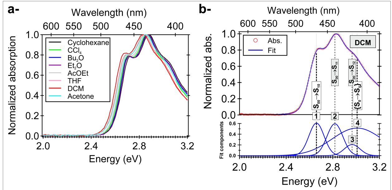
FIG. 12. (Color online) a- Normalized absorption spectra of Curc-di(CN) in various solvents. b- Normalized absorption spectrum of Curc-di(CN) in DCM and corresponding fit with four transitions. The first three are tracing a \pi - \pi^* transition ( S_{00} \rightarrow S_{10} ) and vibronic replicas ( S_{00} \rightarrow S_{11} and S_{00} \rightarrow S_{12} ). The fourth, broad, one labelled \{S_0 \rightarrow S_{ij}\} is ascribed to a set of transitions whose detailed structure is not resolved, from the S_0 electronic ground state to S_{ij} states, where i > 1 and j \geq 0 (cf. text and table I for details).
