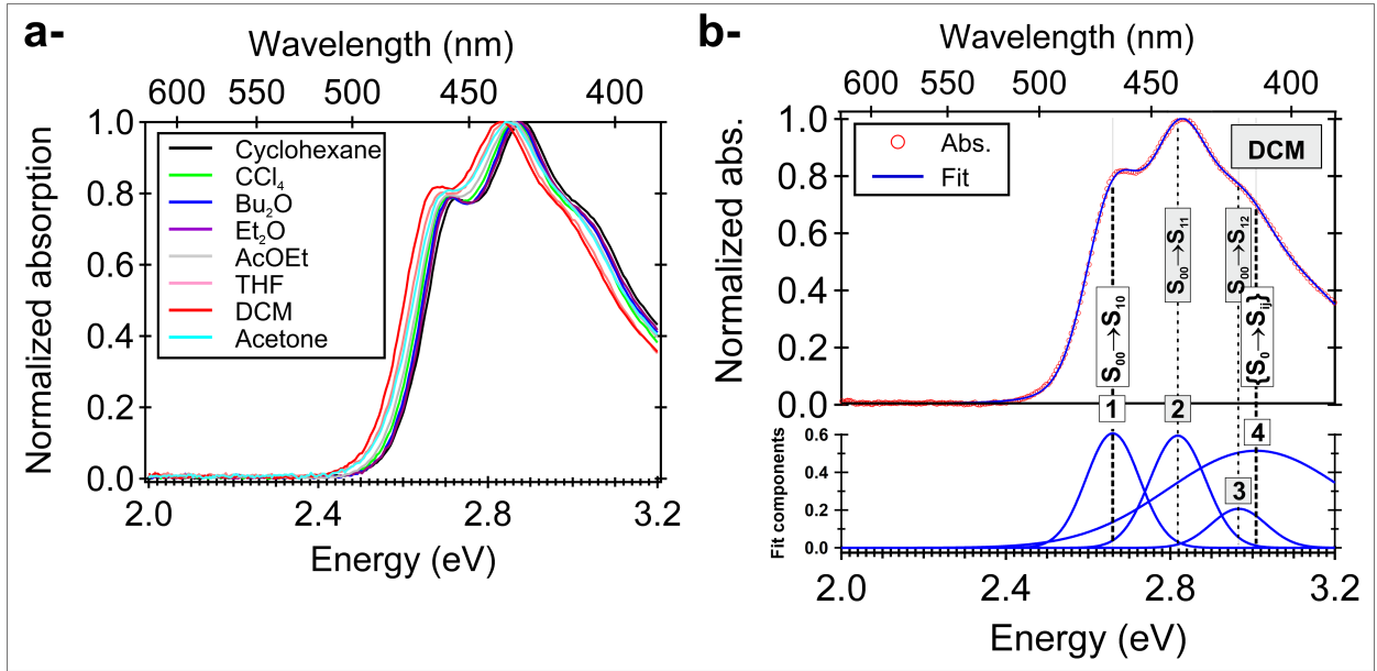
FIG. 12. (Color online) a - Normalized absorption spectra of Curc-di(CN) in various solvents. b - Normalized absorption spectrum of Curc-di(CN) in DCM and corresponding fit with four transitions. The first three are tracing a \pi - \pi^* transition ( S_{00} \rightarrow S_{10} ) and vibronic replicas ( S_{00} \rightarrow S_{11} and S_{00} \rightarrow S_{12} ). The fourth, broad, one labelled \{S_0 \rightarrow S_{ij}\} is ascribed to a set of transitions whose detailed structure is not resolved, from the S_0 electronic ground state to S_{ij} states, where i > 1 and j \geq 0 (cf. text and table I for details).
