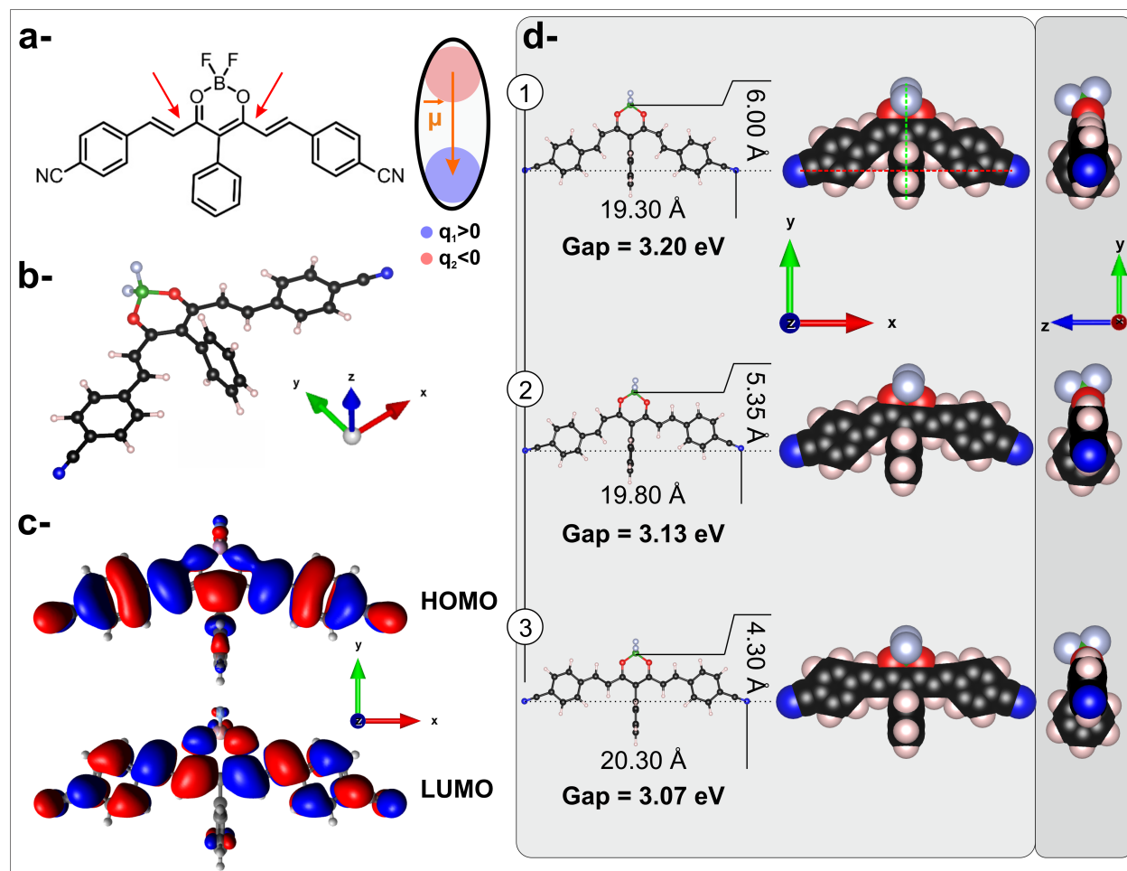
FIG. 1. (Color online). a - Scheme of the Curc-di(CN) molecule. The red arrows indicate the bonds around which the ethylenic groups can rotate to form stereo isomers (as shown in d -). The orientation of the DFT-calculated internal dipole moment of the molecule (cf. text), of strength \mu , is depicted by the orange arrow. b - Perspective view of the isomer 1 of the molecule, as reported in d -. c - Highest occupied- and lowest unoccupied-molecular orbitals (HOMO and LUMO, respectively) for the isomer 3 shown in d3 -, as calculated by DFT (cf. text). d - Balls and sticks, and space filling models of the relaxed configurations of three isomers of the molecule derived by rotation of the ethylenic moieties with respect to the \sigma bond stressed in a -, as calculated by DFT. The HOMO-LUMO gap has been reported for each isomer. For isomer 1, the long (red-dotted line) and short- (green-dotted line) molecular axes are drawn.
