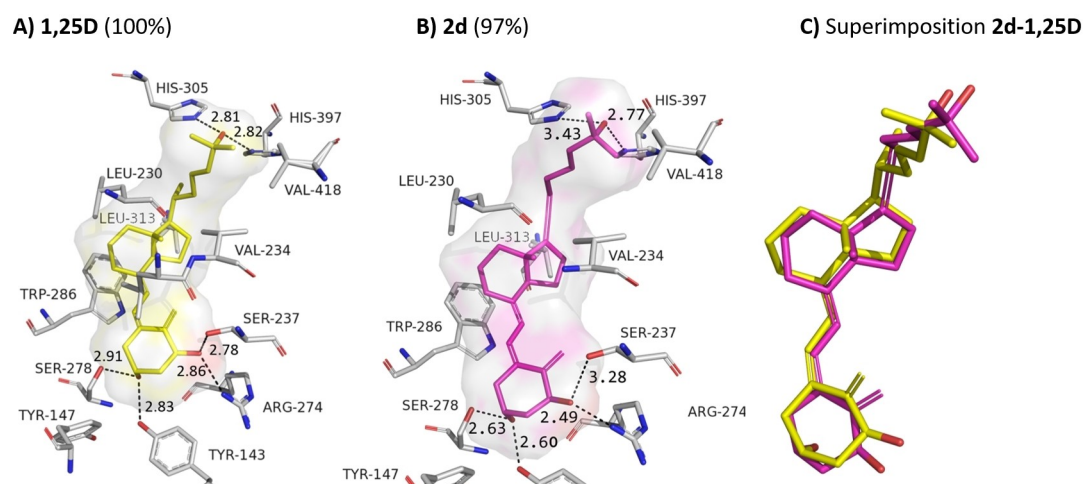
Figure 2. A) Structure of the natural hormone 1,25D (yellow) in complex with hVDR LBD (PDB ID: 1DB1). B) Docked structure of analog 2d (magenta) into the hVDR LBD. C) Superimposition of both 1,25D and 2d . Ligand-amino acid distances are shown in Å.
