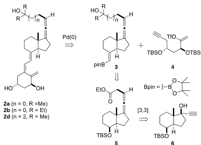
Scheme 1. Retrosynthesis of target analogs 2a , 2b , and 2d from enoltriflate 4 and propargylic alcohol 6 .
