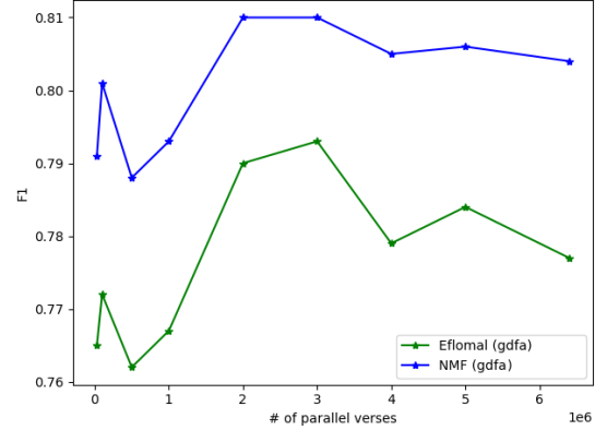
Figure 4: Word alignment F_1 on ENG-FRA as a function of the size of the training set, ranging from 30K to 6.4M training sentence pairs
