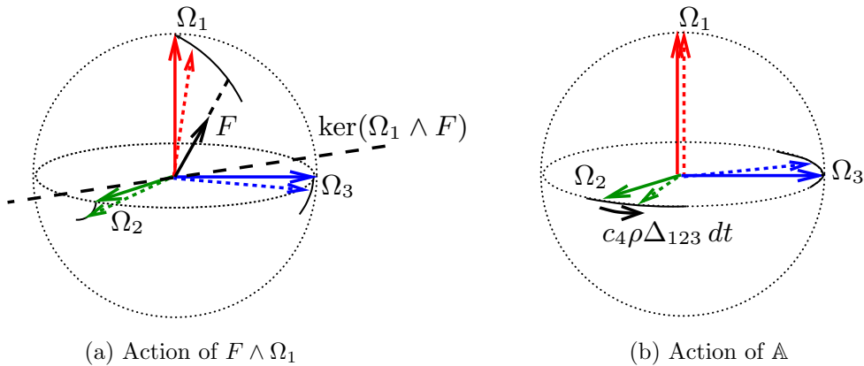
Figure 2: The effects of the two components of \tilde{W} on the motion of the frame, represented in dimension n = 3 by red, green and blue arrows for \Omega_1 (the self-propulsion direction), \Omega_2 and \Omega_3 respectively. The solid arrows represent the frame at a time t and the dashed arrows, at a later time t + \delta t with \delta t \ll 1 . (a) Action of F \wedge \Omega_1 (assuming \mathbb{A} = 0 ): the force F is the black arrow. The frame motion is depicted by the segment of circles joining the ends of the solid arrows and the dashed arrows. The frame rotates in the plane \text{Span}\{F, \Omega_1\} to align \Omega_1 with F . The space (\text{Span}\{F, \Omega_1\})^\perp is the kernel of F \wedge \Omega_1 (the dashed line) so, this space is kept fixed in the frame motion. (b) Action of \mathbb{A} (assuming F = 0 ): the frame rotates about \Omega_1 which remains fixed. Vector \Omega_2 moves in the plane \text{Span}\{\Omega_2, \Omega_3\} with angular speed c_4 \rho \Delta_{123} (and similarly for \Omega_3 ). The displacement of the end of the arrow representing \Omega_2 is depicted by the black arrow.
