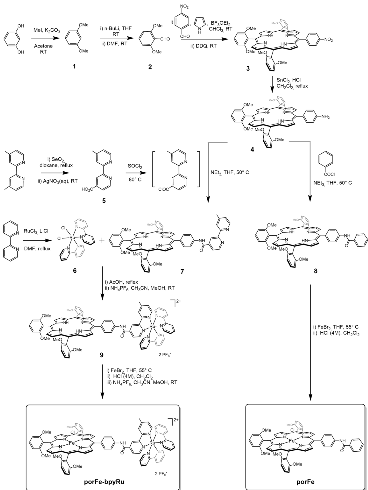
2 Scheme 1. Synthesis of the porFe-bpyRu supramolecular complex and the corresponding reference complex porFe .
