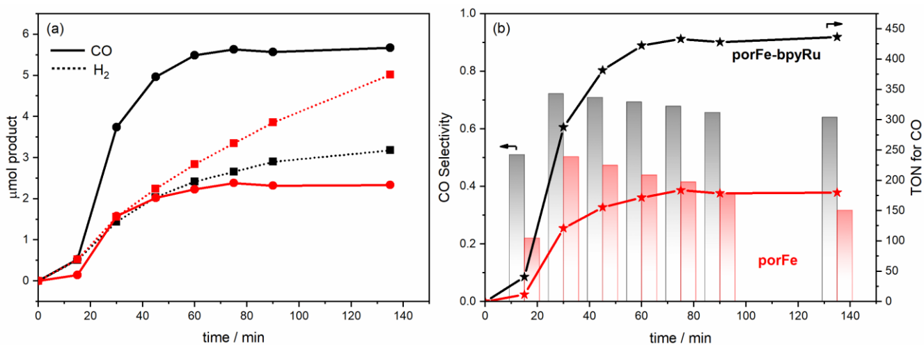
11 12 Fig. 2. (a) Photocatalytic curves for the production of CO (solid lines) and H 2 (dotted lines) during the irradiation of the 13 following in CO 2 -saturated DMF/H 2 O (9:1 v/v): 2 \mu\text{M} porFe-bpyRu + 50 \mu\text{M} bpyRu + 50 mM BIH (black); 2 \mu\text{M} porFe 14 + 50 \mu\text{M} bpyRu + 50 mM BIH (red). (b) Comparison of the photocatalytic performance in terms of selectivity towards CO 15 production (columns) and turnover numbers (TON).
