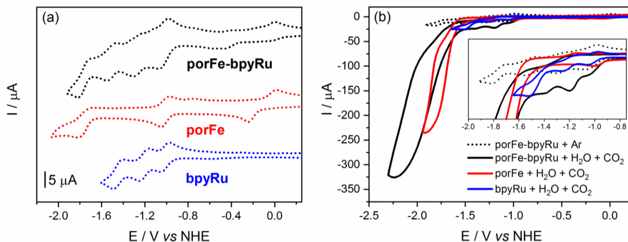
Fig. 1. Cyclic voltammograms (CV) of the supramolecular and reference complexes at concentrations of 0.5 mM in dimethylformamide with 100 mM tetra-N-butylammonium hexafluorophosphate (a) under Ar and (b) under \text{CO}_2 and 5.5 mM \text{H}_2\text{O} . Inset in (b) shows magnification of the onset of catalysis.
