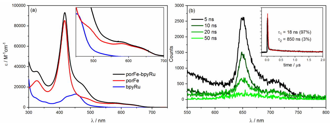
13 14 Fig. 3. (a) Absorption spectra of of the supramoleclar porFe-bpyRu dyad in comparison with the reference complexes in 15 ACN/H 2 O (6:4 v/v). Inset shows magnification of the Q bands region. (b) Transient emission spectra of porFe-bpyRu in 16 DMF upon laser excitation at 460 nm. Inset shows kinetics at 650 nm revealing emission lifetime of 18 ns. Similar transient 17 emission was recorded in ACN/H 2 O (Fig. S2). 18
