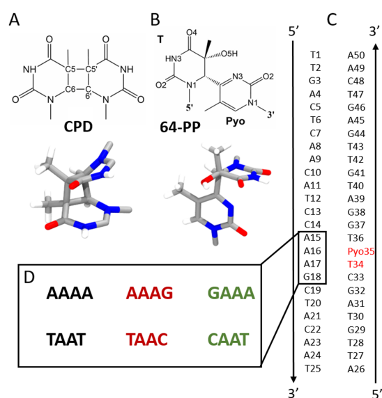
FIG. 1. CPD (A) and 64-PP (B) photolesions in chemical and 3-dimensional representation. C: DNA sequence used in this study, similar to the one from ref 21 . D: six variations on the Watson strands of the flanking pairs of the damage.
