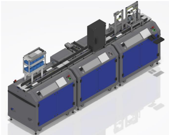
Fig. 7. CAD model (using 3Dx)
