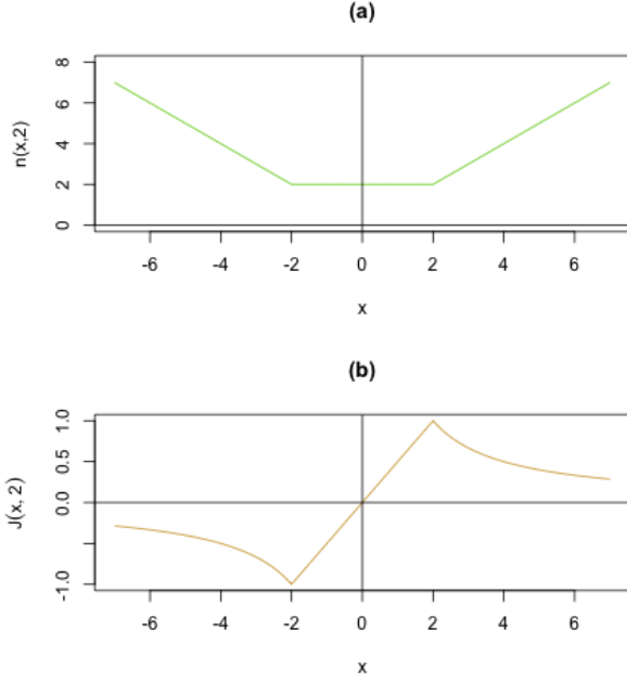
Figure 9: The normalizing function n(x, 2) = \max\{s_x x, 2\} and the normalized operator which corresponds to the real-valued Jaccard index J(x, 2) applied to real scalar values.
