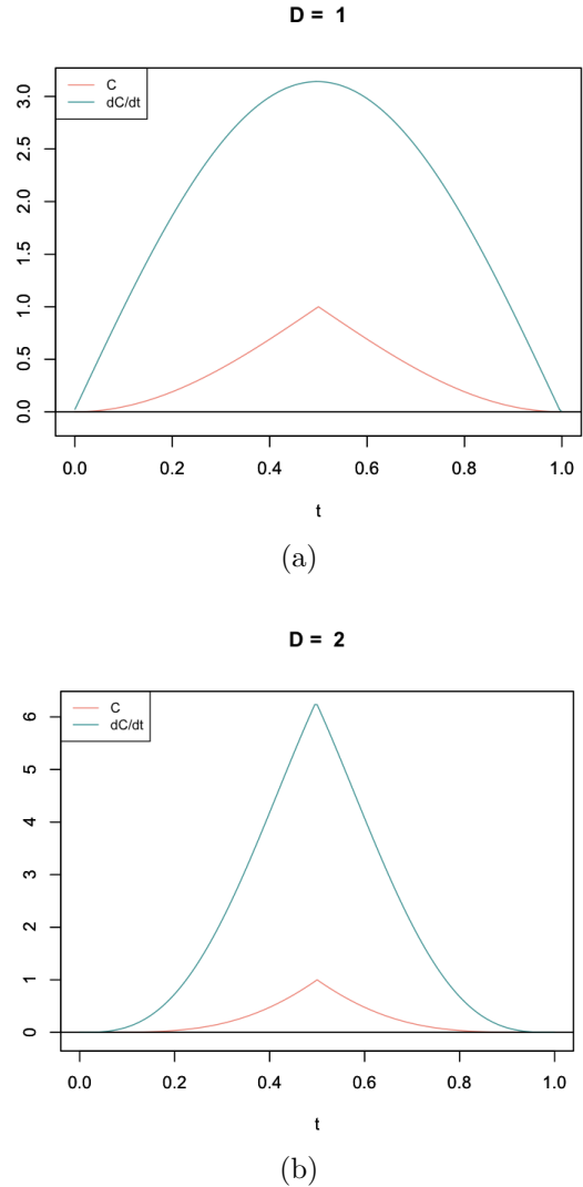
Figure 20: The coincidence similarity values for vector comparisons as in Fig. 4 for D = 1 and D = 2 , and respective derivatives (absolute values). Observe the much sharper derivatives obtained for D = 2 . The region in which the similarity between the two vectors becomes particularly small can be defined with relatively to the values of the respective derivative profile.
