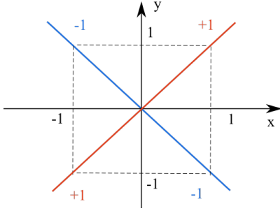
Figure 7: The binary Kronecker function modified to take into account the relative alignment of the real values x and y .
