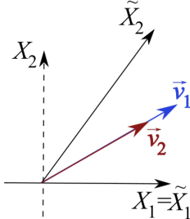
Figure 21: Affine transformations of two similar parallel vectors \vec{v}_1 and \vec{v}_2 cannot change the Jaccard and coincidence similarity.
