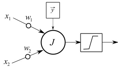
Figure 26: The gemini neuron. The generalization of multiset neurons to incorporate non-linear output function as well as synaptic weights associated to each of its inputs. The comparison part of the neuron can be based on the real-valued Jaccard or coincidence similarities with generic parameter configurations.
