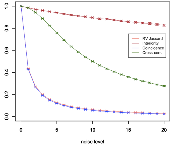
Figure 31: Similarity values obtained by the four considered methods respectively to increasing noise levels. The interiority approach is the most tolerant, followed by the classic cross-correlation, and then the two multiset-based methods. Though these curves correspond to respective averages \pm standard deviations, the latter are generally very small to be visualized.
