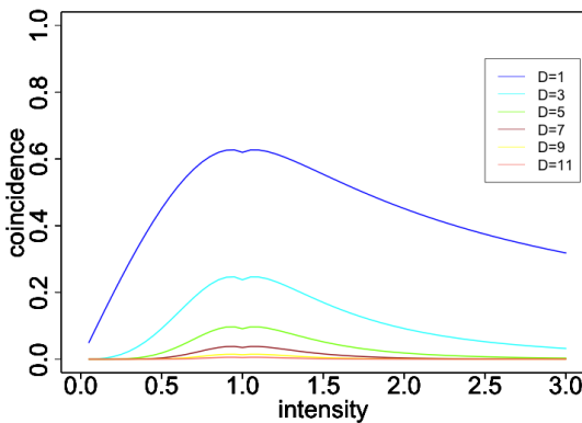
Figure 34: Quantification of the similarity between two circularly symmetric gaussians with the same dispersion, but one of them multiplied by a scaling factor from 0 to 3. The similarity values correspond to the coincidence index for D = 1, 3, 5, 7, 9, 11 .
