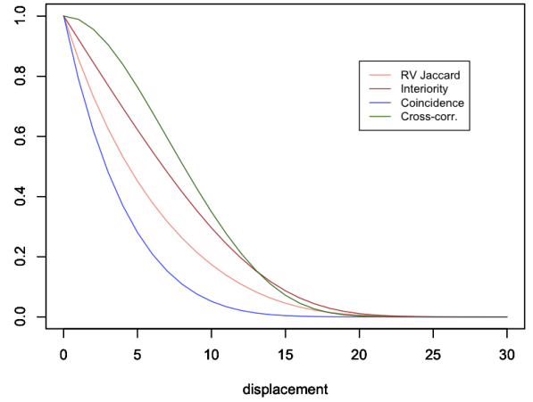
Figure 28: Similarity values obtained by the four considered methods respectively to relative displacements of two identical gaussians. The coincidence method allowed the fastest, and therefore most strict, quantification of the similarity, while the classic cross correlation yielded the most tolerant and least discriminative results.
