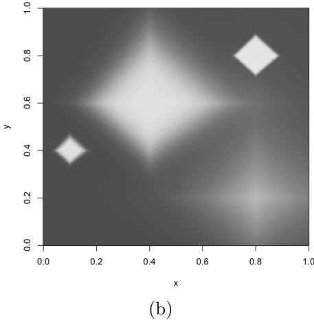
Figure 25: A generalized multiset neuron with N inputs incorporating a non-linear hardlimiting output function, and examples of single neuron 2D receptive fields (b) obtained by varying the sigmoid parameters and template coordinates.
