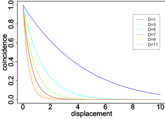
Figure 33: Similarity values obtained by the coincidence similarity for D = 1, 3, 5, 7, 9, 11 respectively to relative displacements of two identical gaussians.
