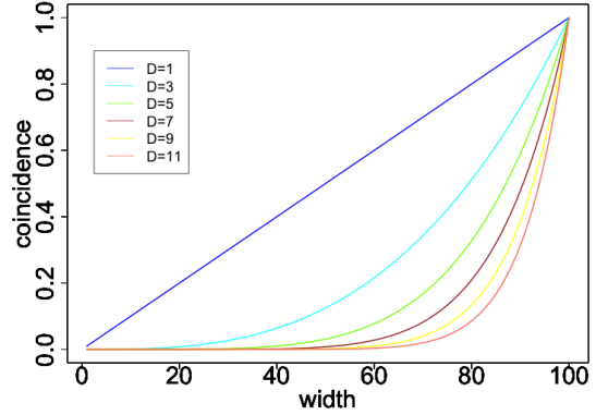
Figure 35: The coincidence similarity between the two patterns in terms of the variation of the width, corresponding to the standard deviation, of one of them.
