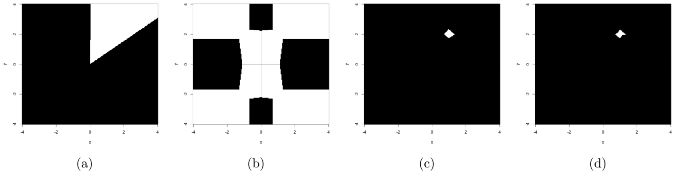
Figure 24: The decision region implemented by the cosine (a), interiority (b), Jaccard (c) and coincidence (d) similarity neurons for similarity values —higher or equal that 0.9 and one of the vectors (template) being equal to [1, 2]^T . The substantially more strict comparison allowed from the Jaccard and coincidence neurons can be readily observed, leading to respectively enhanced pattern differentiation.
