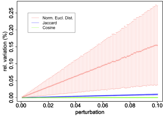
Figure 23: Relative variations of the Jaccard and cosine similarities, as well as the normalized Euclidean distance, to small perturbations of a single component x_i of one of the vectors being compared. Values are shown as average \pm standard deviation, in terms of the magnitude of the individual perturbations. The stabilities of the two similarities, regarding both the average and standard deviations of the relative variations, are substantially smaller than that of the normalized Euclidean distance.
