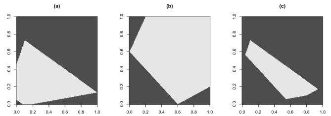
Figure 27: The decision regions (a,b) of two gemini neurons with hard-limit outputs are multiplied in pointwise manner yielding an elaborate decision region which would otherwise require at least 5 more traditional linear discriminant integrate-and-fire neuronal cells.
