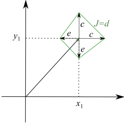
Figure 14: The basic construction characterizing the equisimilarity region for the real-valued Jaccard, defined by the position of vectors \vec{v}_2 = [x_2, y_2]^T when compared to a reference vector \vec{v}_1 = [x_1, y_1]^T and fixed Jaccard similarity value J = d .
