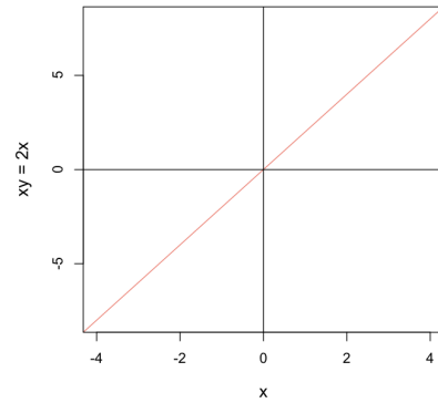
Figure 5: The quantification of similarity between two real values as implemented by the real product xy , with y = 2 has severe limitations. The curve should indicate how similar to 2 the values of x are, but monotonically increasing values are obtained instead.
