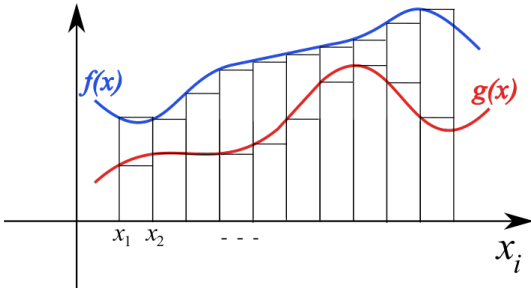
Figure 22: Two functions f(x) and g(x) sampled at equally spaced x_i abscissa values. These two discrete functions can be exactly represented as respective multisets. For simplicity's sake it is assumed that f(x) \geq 0 and g(x) \geq 0 . The common (or shared) area between these two functions is proportional to the multiset intersection between them. The area of the outline of the two functions (maximum values between them) is proportional to the multiset union (e.g. [19, 18]). Though the two functions may intersect one another at several points, for simplicity's sake this is not illustrated in this figure.
