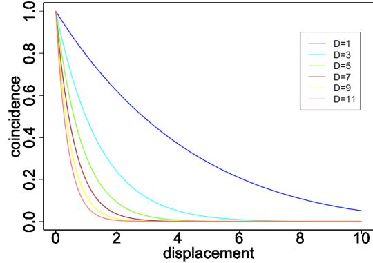
Figure 28: Similarity values obtained by the coincidence similarity for D = 1, 3, 5, 7, 9, 11 respectively to relative displacements of two identical gaussians.
