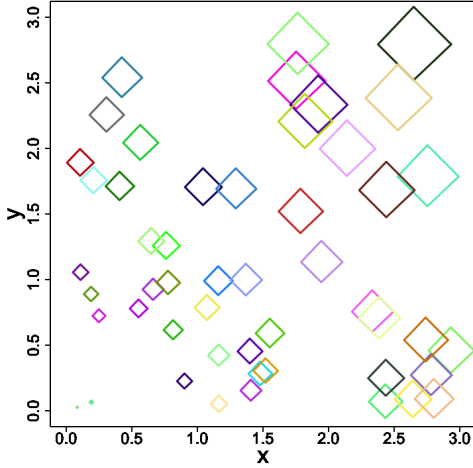
Figure 15: The real-valued Jaccard similarity index is naturally normalized with respect to the scaling of the magnitudes of the compared vectors. This figure illustrates several equisimilarity regions obtained for the real-valued Jaccard similarity with J = d = 0.95 . Observe the linear scale of the regions size with the position of the reference vector.
