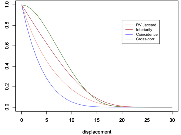
Figure 23: Similarity values obtained by the four considered methods respectively to relative displacements of two identical gaussians. The coincidence method allowed the fastest, and therefore most strict, quantification of the similarity, while the classic cross correlation yielded the most tolerant and least discriminative results.
