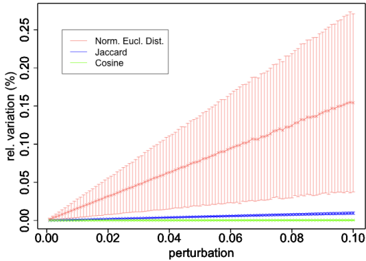
Figure 20: Relative variations of the Jaccard and cosine similarities, as well as the normalized Euclidean distance, to small perturbations of a single component x_i of one of the vectors being compared. Values are shown as average \pm standard deviation, in terms of the magnitude of the individual perturbations. The stabilities of the two similarities, regarding both the average and standard deviations of the relative variations, are substantially smaller than that of the normalized Euclidean distance.
