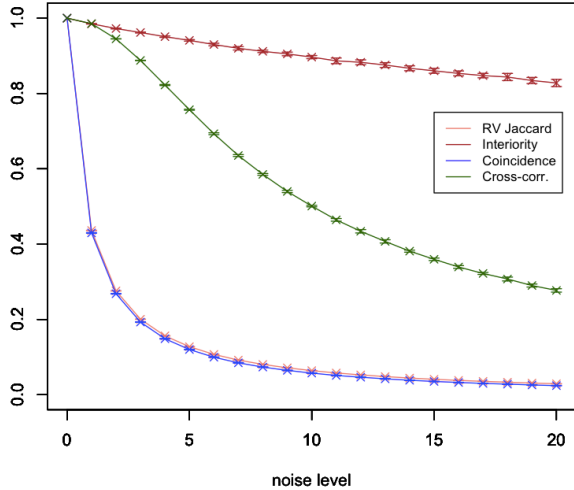
Figure 26: Similarity values obtained by the four considered methods respectively to increasing noise levels. The interiority approach is the most tolerant, followed by the classic cross-correlation, and then the two multiset-based methods. Though these curves correspond to respective averages \pm standard deviations, the latter are generally very small to be visualized.
