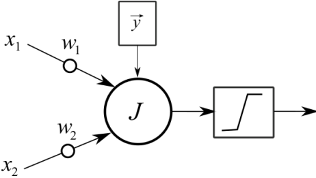
Figure 22: The gemini neuron. The generalization of multiset neurons to incorporate non-linear output function as well as synaptic weights associated to each of its inputs. The comparison part of the neuron can be based on the real-valued Jaccard or coincidence similarities with generic parameter configurations.
