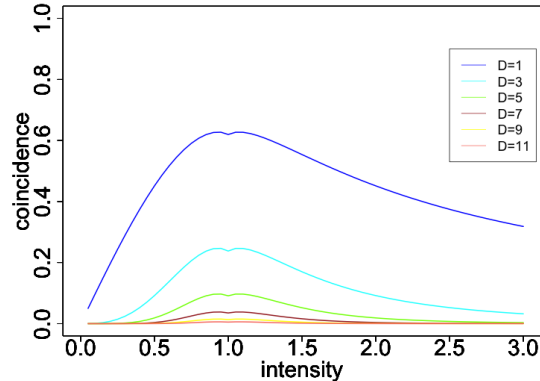
Figure 29: Quantification of the similarity between two circularly symmetric gaussians with the same dispersion, but one of them multiplied by a scaling factor from 0 to 3. The similarity values correspond to the coincidence index for D = 1, 3, 5, 7, 9, 11 .
