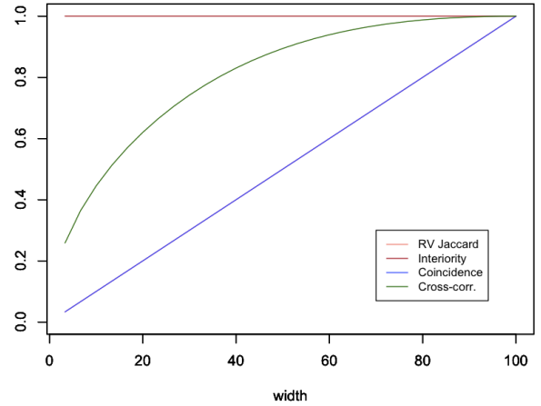
Figure 25: The similarity between the two patterns in terms of the variation of the width, corresponding to the standard deviation, of one of them. The similarity for the real-time Jaccard and coincidence approaches varies linearly from 0 to 1. The cross correlation presents a steep initial variation followed by a saturation. The kept constant at 1, which is expected given that one of the patterns is always interior to the other.
