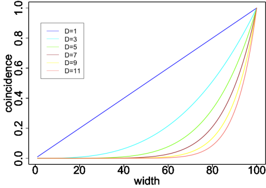
Figure 30: The coincidence similarity between the two patterns in terms of the variation of the width, corresponding to the standard deviation, of one of them.
