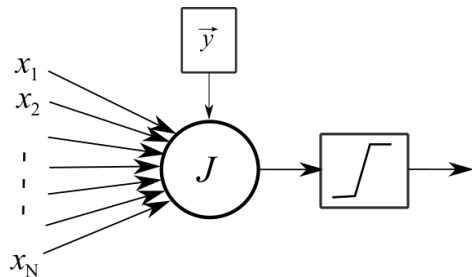
Figure 21: A generalized multiset neuron with N inputs incorporating a non-linear hardlimiting output function.
