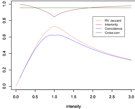
Figure 24: Quantification of the similarity between two circularly symmetric gaussians with the same dispersion, but one of them multiplied by a scaling factor from 0 to 3. In order to impose a more challenging demand, one of the gaussians was always shifted by 2 pixels along each axis. The best results are again observed for the coincidence method, followed by the real-valued Jaccard and interiority approaches. The classic cross correlated revealed to be completely insensitive to the intensity changes.
