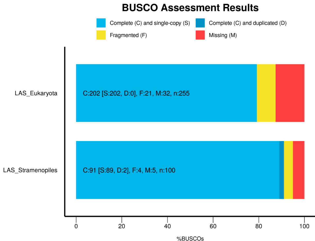
Figure A1. Results of the BUSCO analysis highlighting the presence of complete and single copy Eukaryotic and Stramenopiles genes in the assembly. Letters indicate the BUSCO categories presented in the figure, numbers indicate the number of genes composing a category. ‘n’ indicates the total number of genes in all BUSCO categories.
