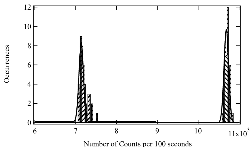
Figure 8: Count distributions obtained for (left) neat water and (right) 5 mM Adenine aqueous solution.
