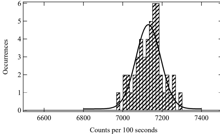
Figure 1: Histogram of the HRS intensity counts per 100 seconds for 47 intervals of equal 300 seconds duration. The full line is a Gaussian fit.
