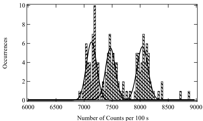
Figure 4(a): Count distributions obtained for the HRS intensity for (left) neat water, (Center) 5mM and (Right) 10 mM Thymine aqueous solutions. See text for the experimental conditions.
