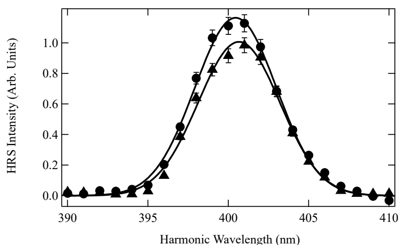
Figure 5: Neat Water (full triangles) and a 10 mM Cytosine aqueous solution (disks) HRS line for a 800 nm fundamental excitation. Corresponding Gaussian fits are provided as full lines. Neat water HRS intensity maximum is normalized to unity.
