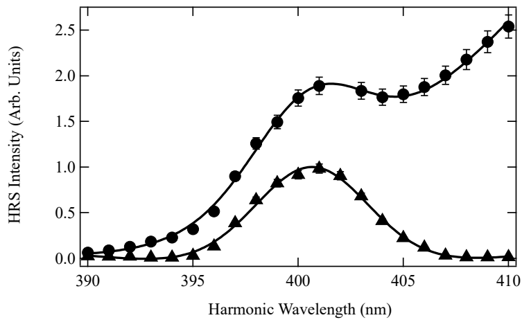
Figure 7: Neat Water (triangles) and a 5 mM Adenine aqueous solution (disks) HRS line for a 800 nm fundamental excitation. Corresponding Gaussian fits are provided as full lines. Neat water HRS intensity maximum is normalized to unity.
