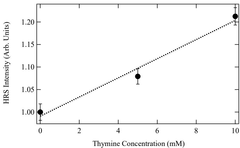
Figure 4(b): Average HRS intensity as a function of Thymine Concentration. Error bars correspond to standard deviation of the adjustment procedure.
