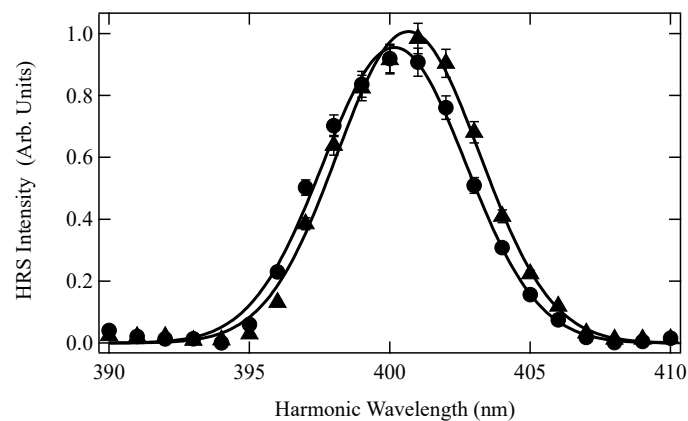
Figure 3: Neat Water (triangles) and a 10 mM Thymine aqueous solution (disks) HRS line for a 800 nm fundamental excitation. Corresponding Gaussian fits are provided as full lines. Neat water HRS intensity maximum is normalized to unity.
