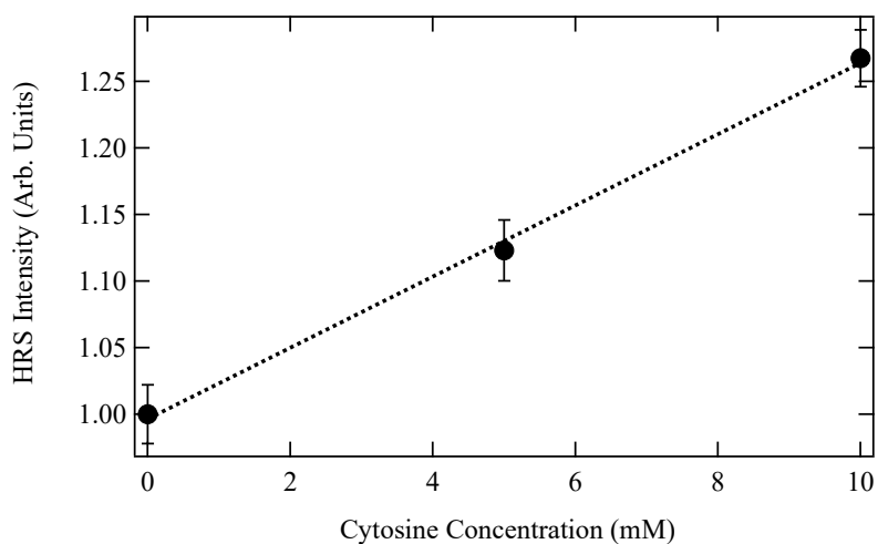
Figure 6(b): Average HRS intensity as a function of Cytosine Concentration. Error bars correspond to standard deviation of the counting procedure.
