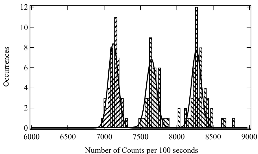
Figure 6(a): Count distributions obtained for the HRS intensity for (left) neat water, (Center) 5mM and (Right) 10 mM Cytosine aqueous solutions.
