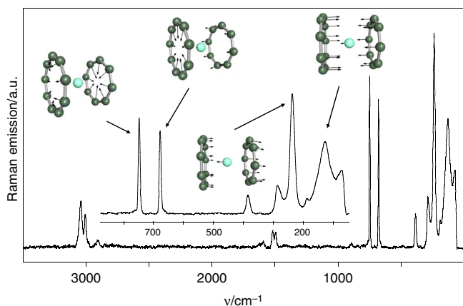
Fig. 6 Raman-spectroscopic analysis. FT-Raman spectrum of [(\eta^9\text{-C}_9\text{H}_9)\text{Sm}(\eta^8\text{-C}_8\text{H}_8)] 3b . The motion vectors of four prominent bands are inserted. Hydrogen atoms and their motion vectors are omitted for clarity
