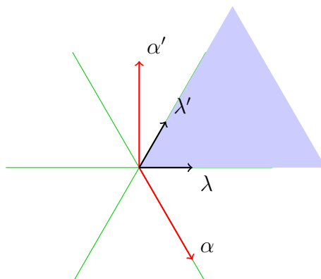
FIGURE 7. A_2 root system
