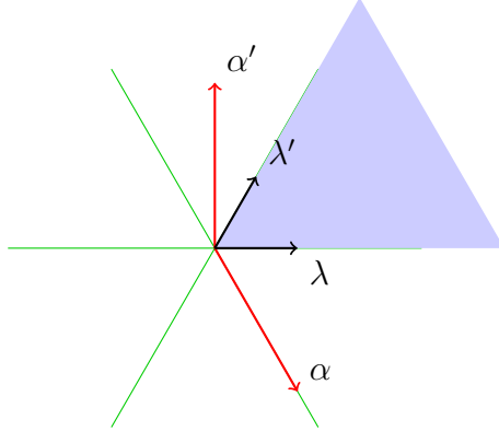
FIGURE 7. A_2 root system
