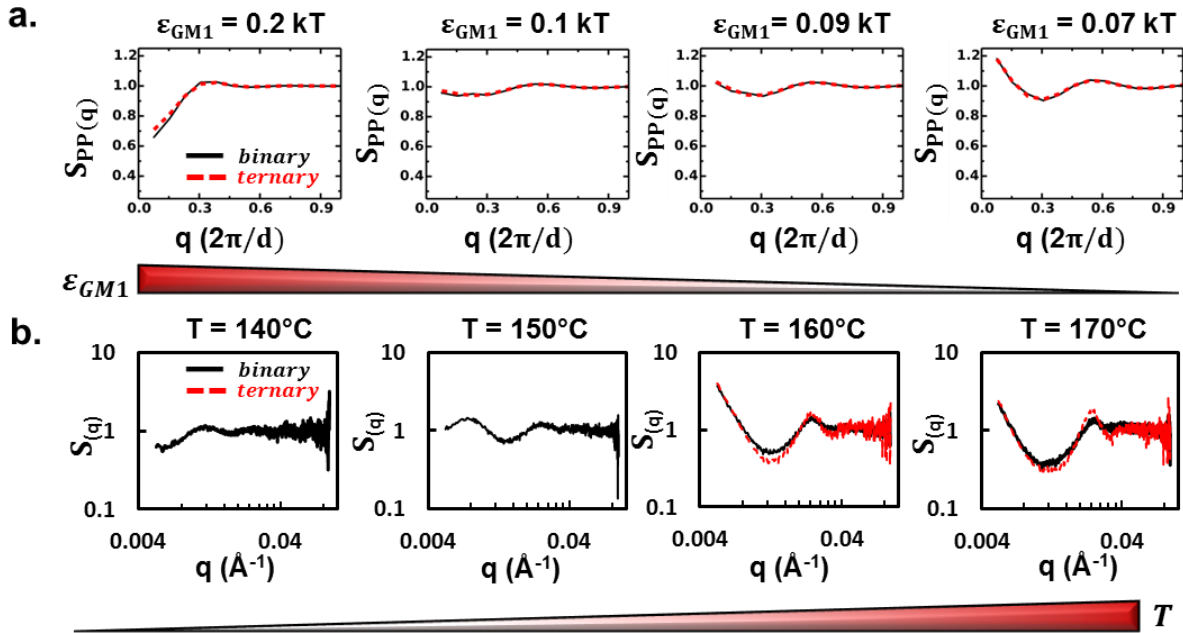
Figure 7. Particle-particle structure factors, S_{pp}(q) , obtained using PRISM theory for PNCs with \phi_{PGP} = 0.039 (a) with \epsilon_{GM1} = 0.2 kT, \epsilon_{GM1} = 0.1 kT, \epsilon_{GM1} = 0.09 kT and \epsilon_{GM1} = 0.07 kT. Figure 7b shows the corresponding particle-particle structure factors, S(q) , obtained using SAXS for 25/75 wt% PNCs. The binary PNC case with \phi_{M2} = 0 is shown as a black line and the ternary case with \phi_{M2} = 0.043 (5 wt%) is shown as a red dashed line. Results in part (a) are obtained using PRISM theory for PNCs with \epsilon_{GG} = \epsilon_{M1M1} = 0.1 kT, D_p = 5d , N_G = 15 , N_{M1} = 75 , N_{M2} = 15 , \Sigma = 0.76 chains/ d^2 .
