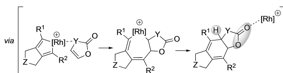
Scheme 25. Formal cross-alkyne cyclotrimerisation reaction using vinylene carbonate and 2-oxazolone as alkyne surrogates under rhodium catalysis.
