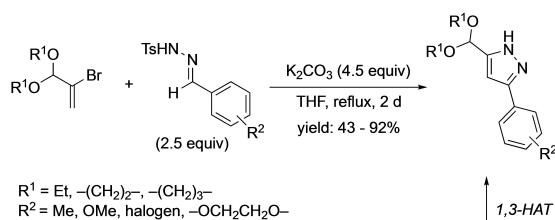
Scheme 1. 1,3-dipolar cycloaddition reaction of N -phenylbenzenehydrazonyl chloride derivatives with \alpha -bromocinnamaldehyde.
