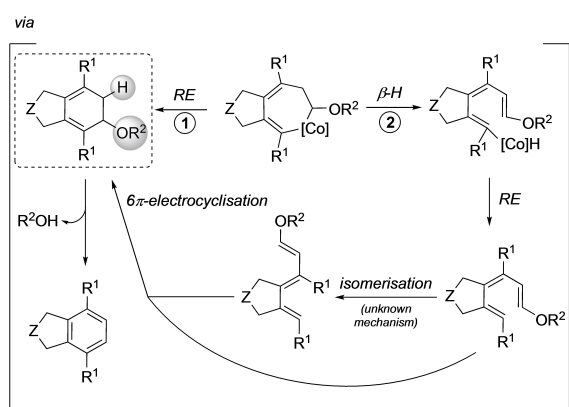
Scheme 22. Formal cross-alkyne cyclotrimerisation reaction using enol ethers as alkyne surrogates under cobalt catalysis.
