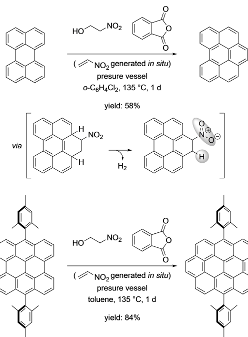
Scheme 13. Diels-Alder cycloaddition/aromatization sequence for the controlled synthesis of CNTs from planar templates.
