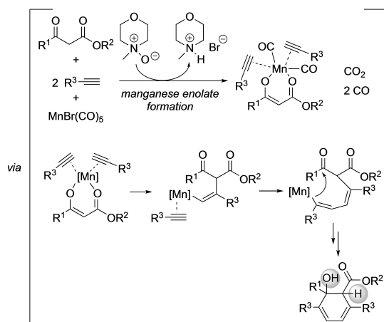
Scheme 23. Formal cross-alkyne cyclotrimerisation reaction using 1,3-dicarbonyl derivatives as alkyne surrogates under manganese catalysis.
