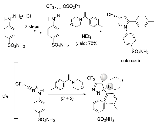
Scheme 5. Total synthesis of celecoxib.
