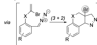
Scheme 3. Synthesis of dihydrobenzopyrano- and dihydroquinolinopyrazoles via an intramolecular 1,3-dipolar cycloaddition reaction.
