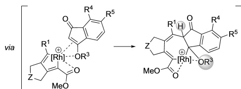
Scheme 26. Formal cross-alkyne cyclotrimerisation reaction using 3-acetoxy and 3-alkoxyindenes as cycloalkyne surrogates under rhodium catalysis.
