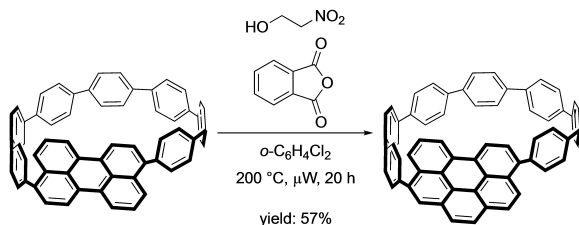
Scheme 14. Diels-Alder cycloaddition/aromatization sequence for the controlled synthesis of CNTs from macrocyclic curved template.
