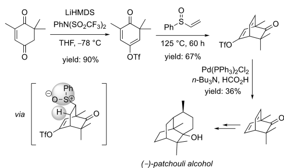
Scheme 19. Diels-Alder cycloaddition/elimination sequence for the synthesis of benzo[d]isothiazole-1,1-dioxide core.
