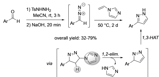
Scheme 6. One-pot, three-steps procedure for the regioselective preparation of 3-substituted pyrazoles.
