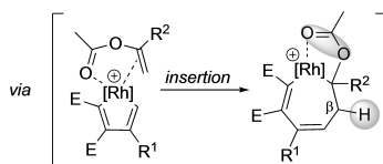
Scheme 21. Formal cross-alkyne cyclotrimerisation reaction using enol ethers and vinylic acetates as alkyne surrogates under rhodium catalysis.
