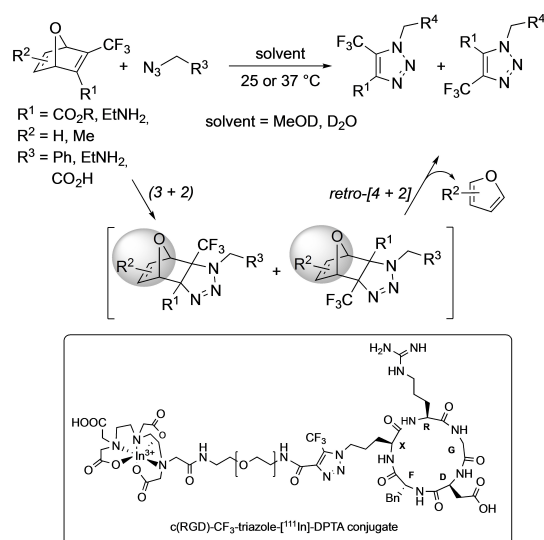
Scheme 10. Metal-free triazole synthesis as a tool for bioconjugation.
