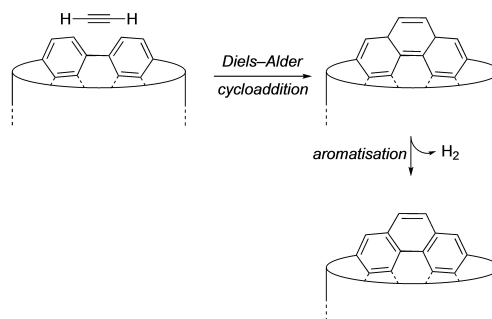
Scheme 12. Diels-Alder cycloaddition/aromatisation sequence for the controlled synthesis of CNTs.
