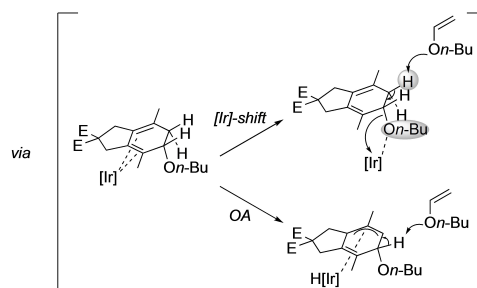
Scheme 20. Formal and partially intramolecular cross-alkyne cyclotrimerisation reaction using enol ethers as alkyne surrogates under iridium catalysis.
