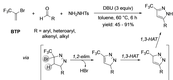
Scheme 4. Synthesis of 3-trifluoromethylpyrazoles by a multicomponent process.
