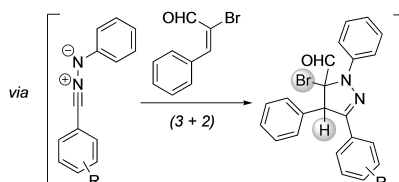
Scheme 1. 1,3-dipolar cycloaddition reaction of N -phenylbenzenehydrazonyl chloride derivatives with \alpha -bromocinnamaldehyde.
