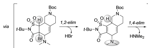
Scheme 18. Diels-Alder cycloaddition/double elimination sequence for the synthesis of benzo[d]isothiazole-1,1-dioxide core.
