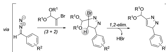
Scheme 2. 1,3-dipolar cycloaddition reaction of in situ generated diazo intermediates with \alpha -bromovinylacetals.
