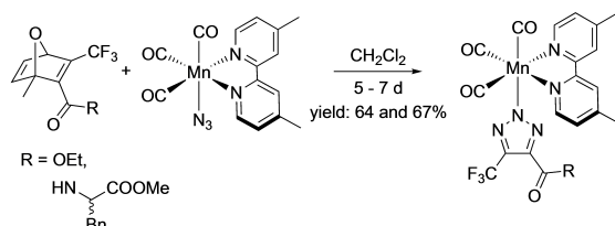
Scheme 11. Biorthogonal coupling reactions.
