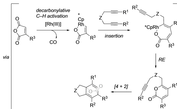
Scheme 16. Formal [2+2+2] cycloaddition using maleic anhydrides as alkyne equivalents for the synthesis of benzene derivatives.
