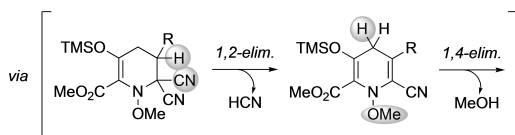
Scheme 17. Diels-Alder cycloaddition/aromatization sequence for the synthesis of substituted 3-hydroxypyridines.
