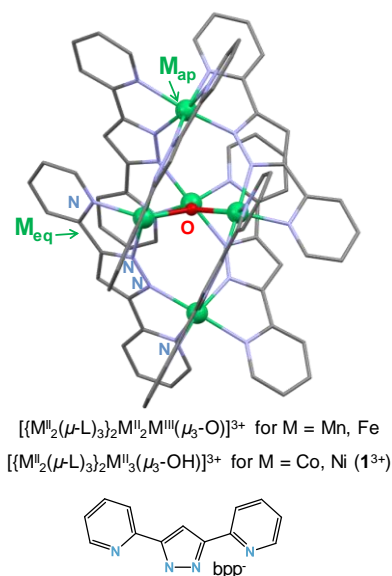
Scheme 1. Schematic representation of the molecular structure of the \{[M(\mu\text{-bpp})_3]_2M_3(\mu_3\text{-X})\}^{n+} complexes ( M_{ap} and M_{eq} refer to metal M located in apical and in equatorial position, respectively) and of the deprotonated bpp - ligand.
