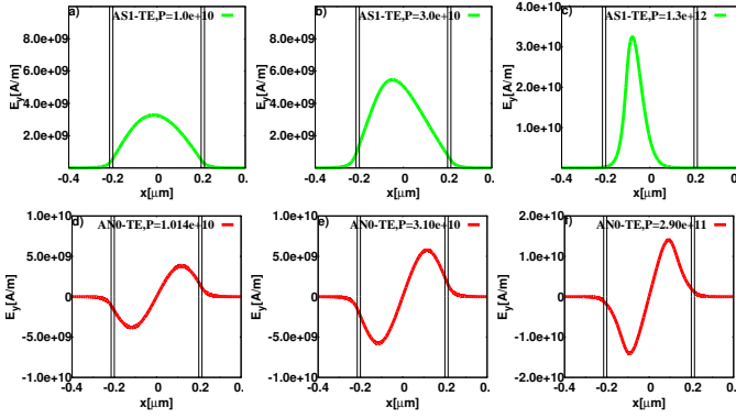
FIG. 16. Nonlinear field profiles E_y(x) for the improved NPSW in the TE case. The top green curves and the bottom red curves for ASI-TE and AN0-TE, respectively, with d_{core} = 400 nm, \varepsilon_{buf} = 2.5^2 , and d_{buf} = 15 nm. The power is given in W/m.
