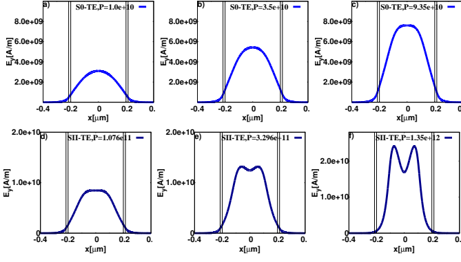
FIG. 15. Spatial transition of the symmetric nonlinear field profiles E_y(x) for the improved NPSW in the TE case. (top) for S0-TE and (bottom) for SII-TE with d_{core} = 400 nm, \varepsilon_{buf} = 2.5^2 , and d_{buf} = 15 nm. The power is given in W/m.
