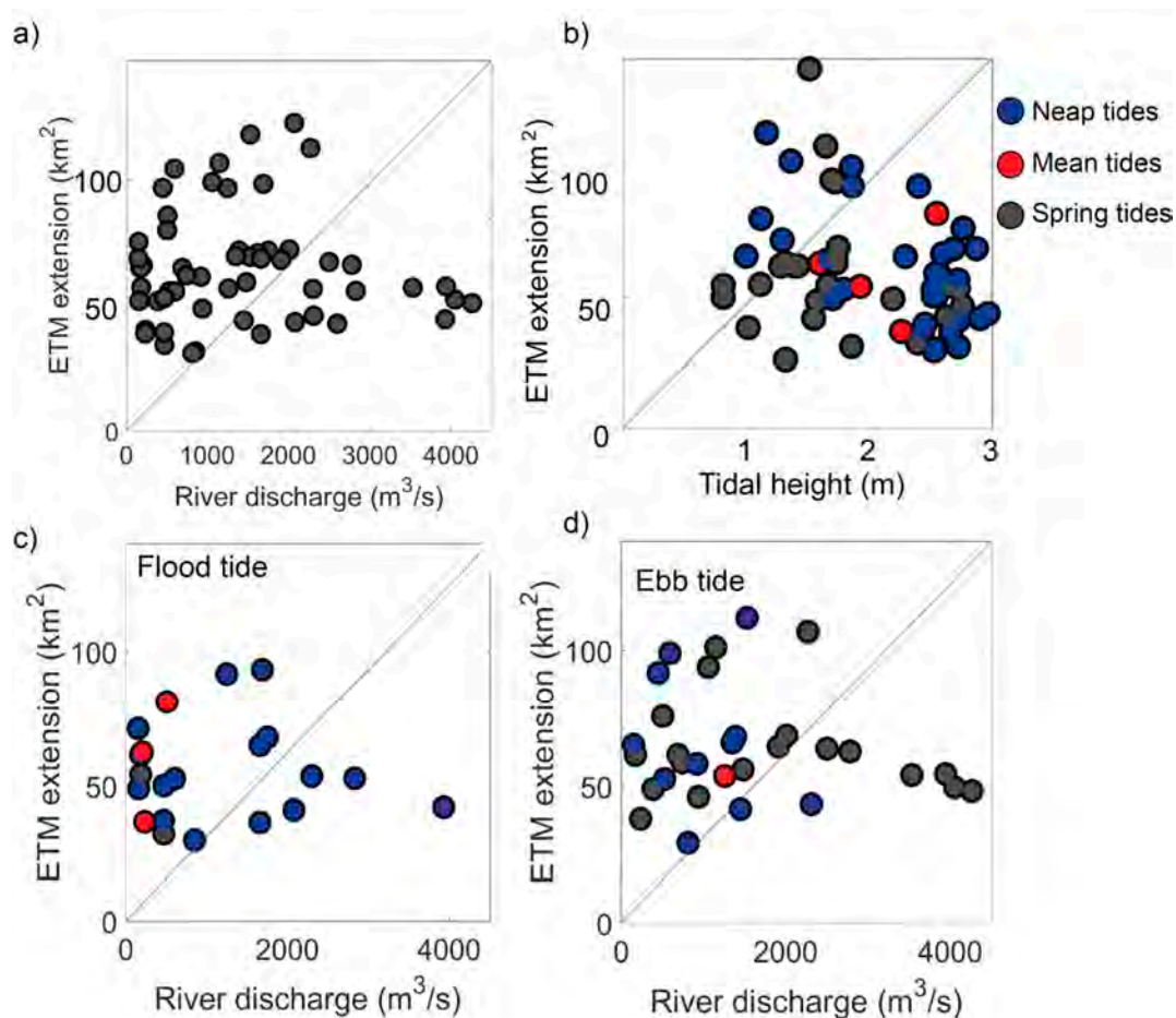
Figure 7. Comparison of the ETM extension (in \text{km}^2 ) with two dynamic drivers, river discharge and tides. (a) ETM extension and river discharge. (b) ETM extension and tidal height values for all tides. Blue dots correspond to images characterized by neap tides, red dots by mean tides and grey dots by spring tides as explained in Section 2.2.5. (c) ETM extension compared to flow rate values for those images presenting flood tide and (d) compared to those images presenting ebb tide.
