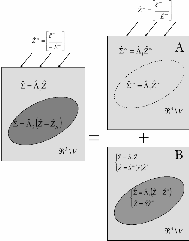
Fig. 2 Scheme describing the Eshelby equivalence principle applied to the case of a piezoelectric matrix. The problem A corresponds to a uniform medium \hat{\Lambda}_1 with remotely applied fields \vec{E}^\infty and \hat{\epsilon}^\infty . In such a case we observe that the fields remain uniform in the entire space. The problem B represents an inclusion problem with eigenfield \hat{Z}^* and without external actions. In this case the generalized strain and stress are given by \hat{Z} = \hat{S} \hat{Z}^* and \hat{\Sigma} = \hat{\Lambda}_1 (\hat{S} - \hat{I}) \hat{Z}^* , as predicted by the Eshelby theory. The superimposition of the two sub-problems allows us to solve the original problem of the particle described by \hat{\Sigma} = \hat{\Lambda}_2 (\hat{Z} - \hat{Z}_\mu) embedded in the piezoelectric matrix.
