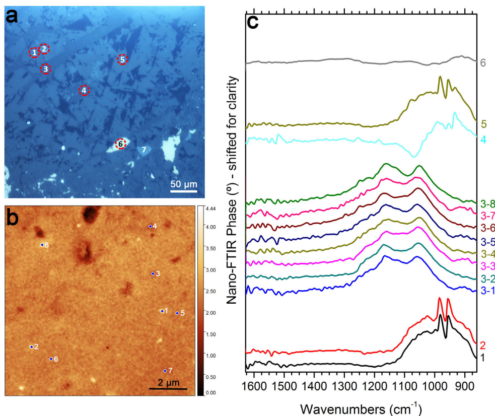
Fig. 9. a) Visible light image of Location III. The studied spots are indicated by a red dashed circle. b) AFM image of spot 3. Measured points in this spot are numbered from 1 to 8. c) Nano-FTIR spectra of corresponding spots and points. Olivine has a distinct spectra (such as spectra 1 and 2). Feldspar is characterized by two strong and a weak shoulder band (all spectra in spot 3). Spectrum 6 is due to an opaque metallic phase. (Color figure can be viewed at wileyonlinelibrary.com .)
