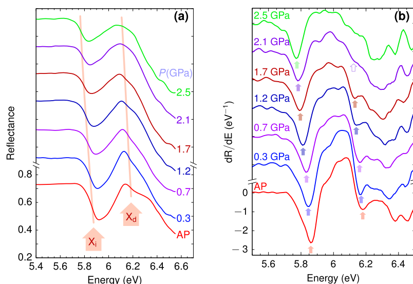
Figure 1. (a) Reflectance spectra of h -BN for pressures up to 2.5 GPa. The traces have been vertically shifted by 0.2 steps for clarity. The vertical lines indicate the shift with pressure of the features associated with the direct ( X_d ) and indirect ( X_i ) excitonic transitions. (b) Derivative of the reflectance spectra. The traces have been vertically shifted for clarity. The arrows indicate the minima of dR/dE corresponding to the excitonic transition.
