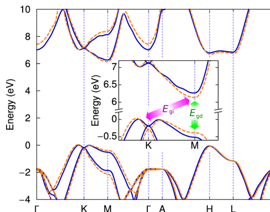
Figure 4. Electronic band structure calculated at the GW level. Solid lines are ambient pressure results, and dashed lines correspond to a hydrostatic pressure of 2.5 GPa. Inset: blow-up view of the band structure in the region of the indirect and direct bandgaps.
