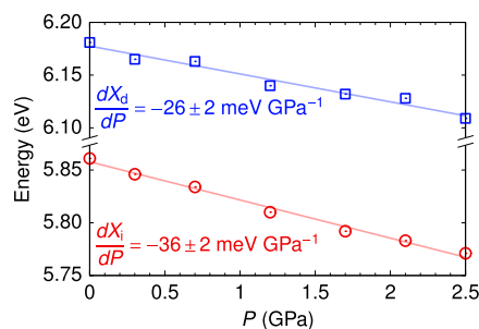
Figure 3. Pressure dependence of the X_d and X_i energies as determined from the reflectance spectra.
