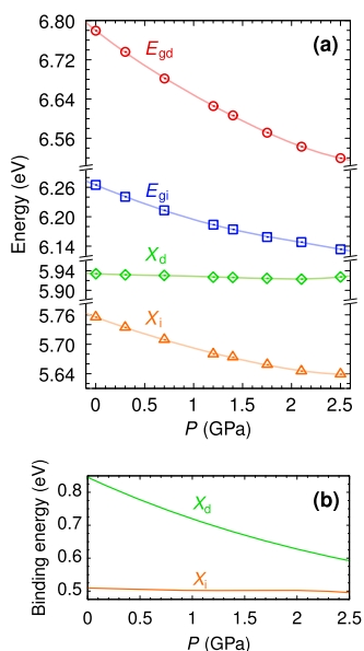
Figure 5. (a) Pressure dependence of the direct and indirect bandgaps and excitonic transitions of h -BN. The direct ( E_{gd} ) and indirect ( E_{gi} ) bandgaps were calculated at the GW level. The direct ( X_d ) and indirect ( X_i ) excitonic transitions were calculated at the ab initio many-body perturbation theory level ( GW and Bethe–Salpeter equation). (b) Exciton binding energies as a function of pressure.
