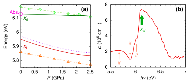
Figure 6. (a) Direct ( X_d , diamonds) and indirect ( X_i , triangles) excitonic transitions determined from the reflectance spectra compared with the ab initio theoretical calculations (solid lines). A rigid shift of 196 meV independent of pressure was applied to the theoretical results to bring them into accordance with the measured peak of the absorption spectrum (magenta circle). The dotted line represents the indirect transition absorption peak taking into account the energy of the ZA/ZO 1 ( T ) assisting phonons. 29 (b) Absorption spectrum at ambient pressure of a very thin h -BN sample ( \sim 50 nm) in the spectral region of the direct excitonic transition. The arrows labeled if indicate structures corresponding to the Fabry–Perot interference fringe pattern of the 50 nm thick sample. The fat arrow indicates the direct excitonic transition.
