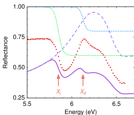
Figure 2. Calculated reflectivity spectrum associated with the direct excitonic transitions (dashed line), compared with the experimental reflectance measurement (red dots). The blue and green sigmoidal dotted lines account for, respectively, the drop of reflectance due to the absorption at the direct and indirect excitonic energies suppressing the reflection at the bottom interface. The solid line is the resulting calculated reflectance after taking into account the self-absorption effect.
