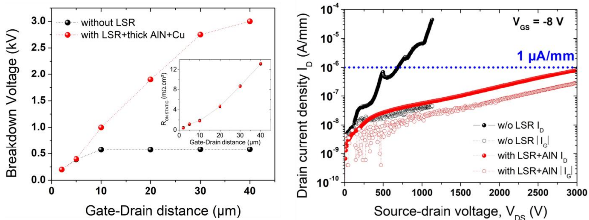
Figure 32: (left) Evolution of LGD-dependent device V_{BR} and specific on-resistance (inset) of AlGaN/GaN HEMTs with and without LSR by defining the blocking voltage at I_D = 1 \mu\text{A/mm} , and (right) off-state leakage current characteristics of AlGaN/GaN MISHEMTs with and without LSR. Reprinted from "GaN-on-silicon high-electron-mobility transistor technology with ultra-low leakage up to 3000 V using local substrate removal and AlN ultra-wide bandgap", Ezgi Dogmus et al., Appl. Phys. Express, https://doi.org/10.7567/APEX.11.034102 , licensed under CC BY 4.0 [25].
