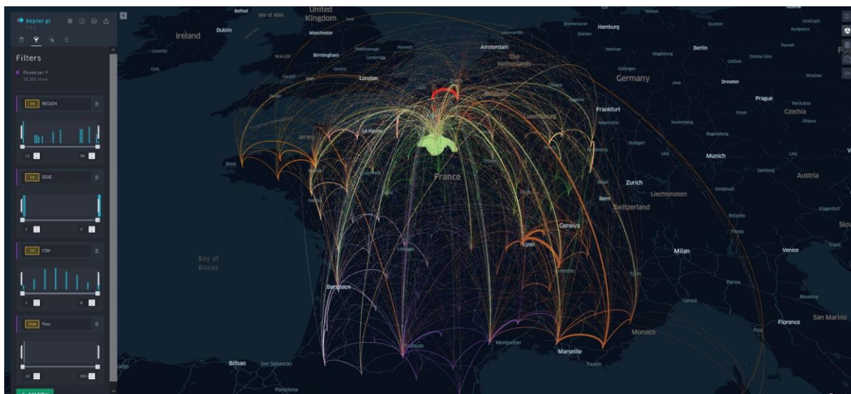
Figure 4. Kepler.gl interface
