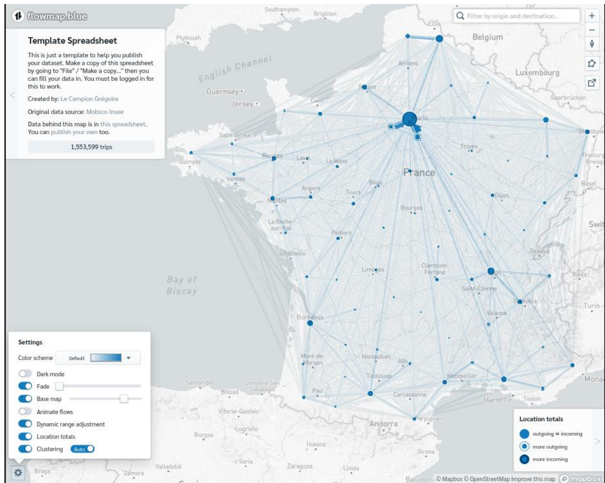
Figure 5. Flowmap.blue interface
