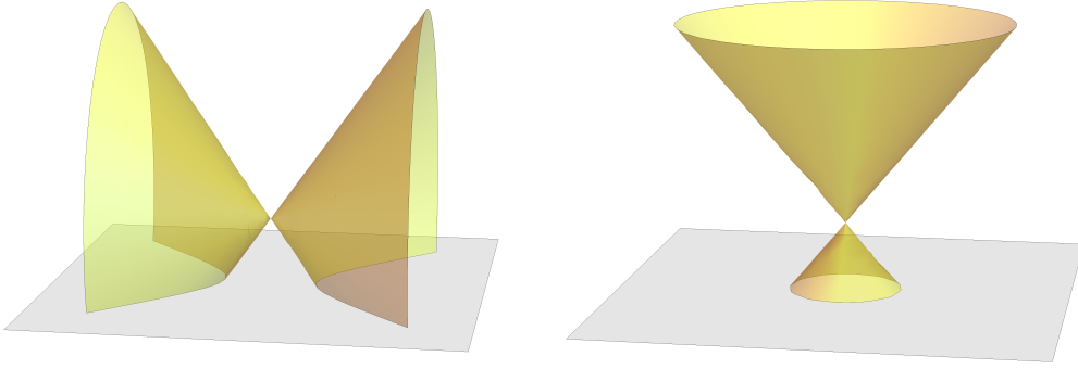
FIGURE 2. The lightcone from a point in \mathcal{H}^{2,1} (left) and \mathcal{H}^{1,2} (right).
