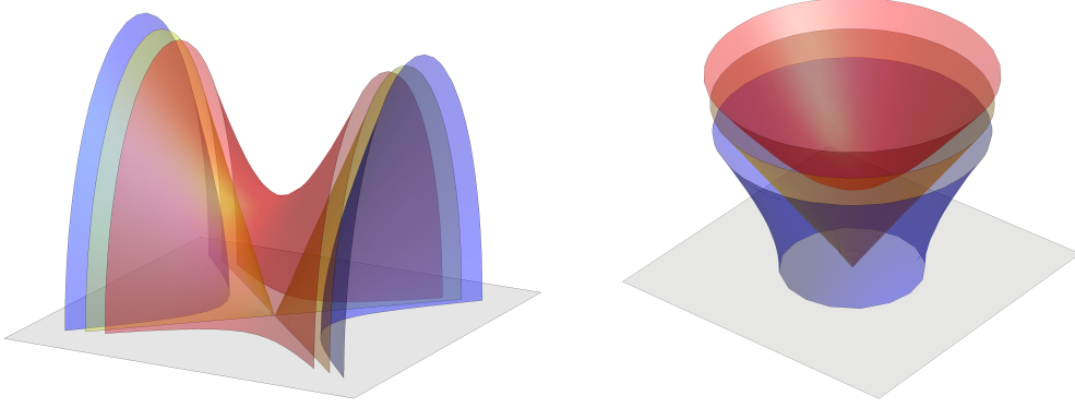
FIGURE 1. The totally geodesic quadric hypersurfaces in \mathcal{H}^{2,1} (left) and \mathcal{H}^{1,2} (right).
