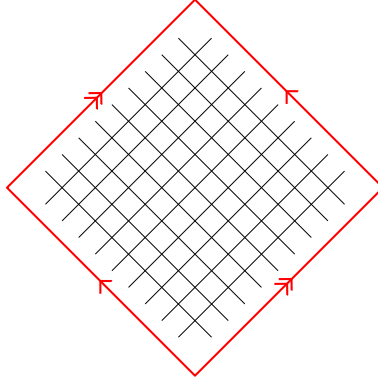
FIGURE 4. The compactification of \partial\mathcal{H}^{2,1} , which is a copy of \mathbb{R}^{1,1} represented by the interior of the diamond, inside \partial_\infty\mathcal{H}^{2,1} . The lines at \pm 45^\circ represent the degenerate affine subspaces in \mathbb{R}^{1,1} , and each of them is compactified to a different point. The point \infty then corresponds to the vertices of the diamond. The identifications of the sides clearly give the topology of a torus on \partial_\infty\mathcal{H}^{2,1} .
