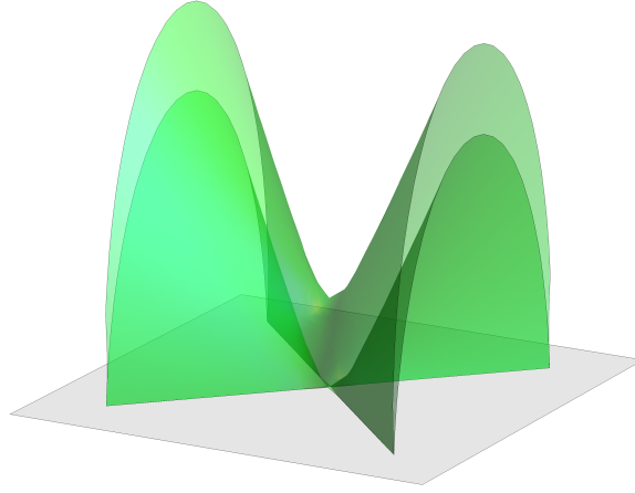
FIGURE 6. Horospheres in \mathcal{H}^{2,1} corresponding to a point in \partial\mathcal{H}^{2,1} .
