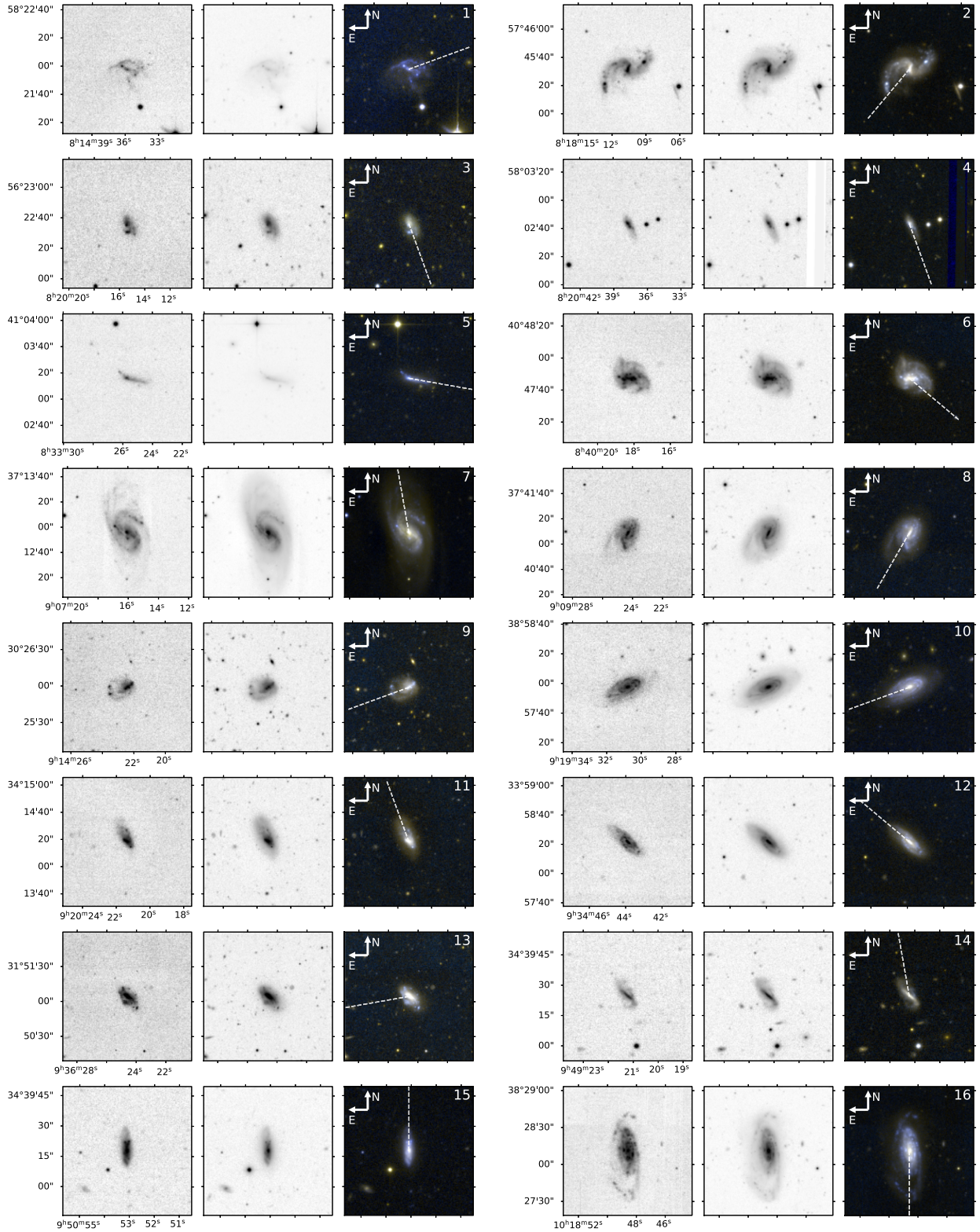
Figure A1. u -band (left), r -band (center), and rgb (right) for the RP candidates identified in this work. White line indicates the estimated 'tail' direction for each RP candidate (see Section 4.2.2).
