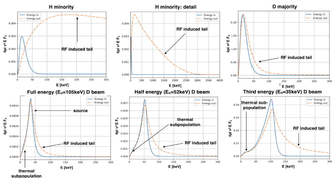
Figure 2 Energy density (distribution function F_0 integrated over gyro and pitch angle, multiplied by the Jacobian in velocity space v^2 and the energy) in the core ( \rho = 13\text{cm} ) for the 5 solved populations (from top left to bottom right): H minority, D majority, D beams (having birth energy = 105, 52, 35 keV) without ICRH (blue curves) and after RF tail has formed (orange dashed). For the fundamental cyclotron heating N=1 the whole distribution is deformed in the thermal region (top left plot, zoom in middle). For second harmonic heating the distribution is mostly deformed by the slowing down energy from the heated subpopulation which adds energy to the thermal region raising the Maxwellian to higher temperature, while a high energy tail is formed.
