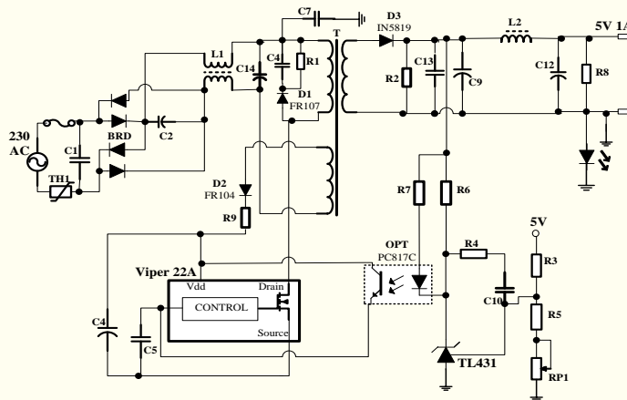
Figure 3. Schematic of the studied flyback AC/DC converter.
