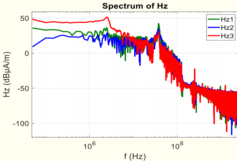
Figure 11. Spectrum of the measured magnetic field above DUT at different positions.
