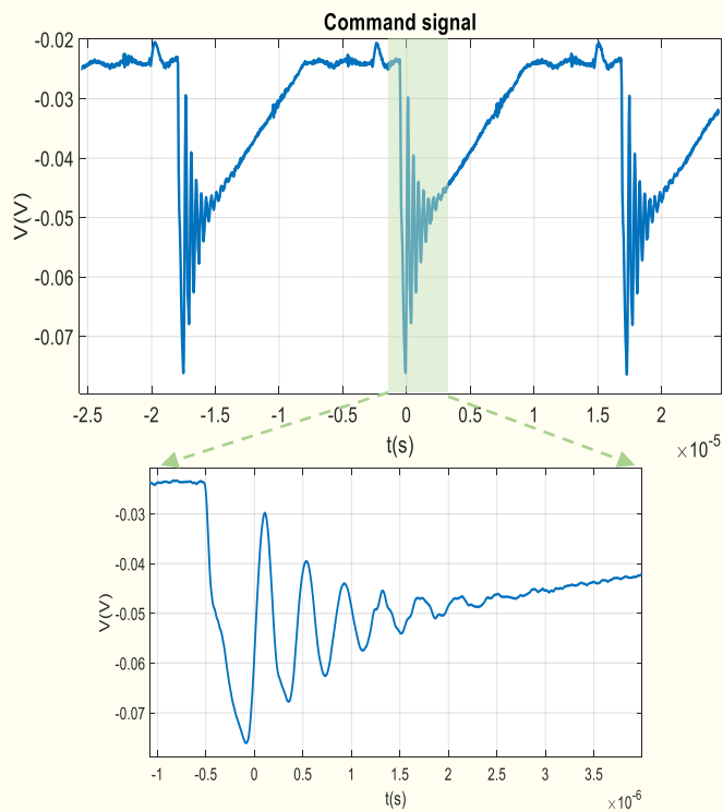
Figure 4. Control signal.
