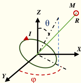
Figure 7. Definition of an equivalent magnetic dipole.
