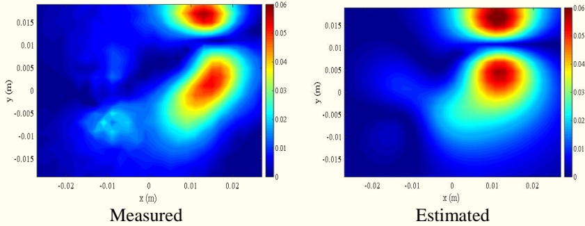
Figure 13. Measured and estimated magnetic NF maps of x -component at t = 10.50 \mu\text{s} .
