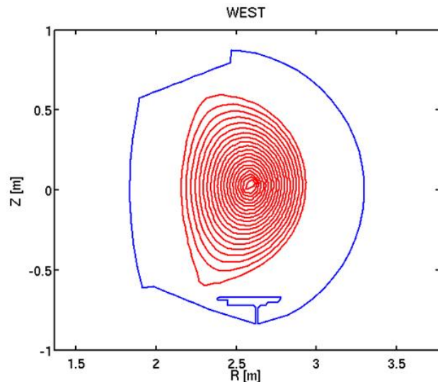
Figure 5: Closed flux surfaces of a WEST plasma equilibrium (red contours) as reconstructed by the EQUINOX code from synthetic magnetics measurements. The blue line is a simplified contour of the surfaces of the in-vessel components closest to plasma.
