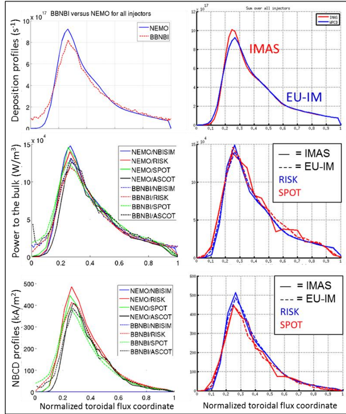
Figure 3: Result of the NBI benchmark using the H&CD workflow in EU-IM (left figures) and IMAS (right figures) frameworks for the ITER baseline scenario for the off-off neutral beam configuration. Top / middle / bottom figures show the deposition profiles, power to the bulk profiles and NBCD profiles respectively.
