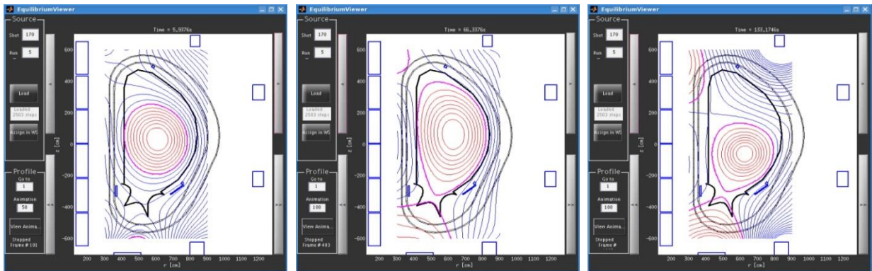
Figure 2: Examples of plasma equilibria at times 5.9s, 66.3s and 133.1s from the IDS database populated from a 280s DINA simulation of ITER
