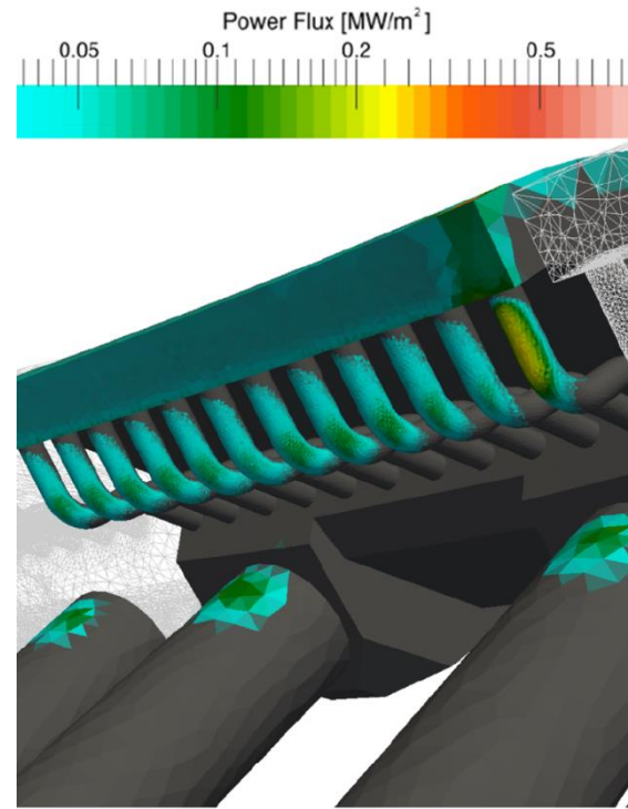
Figure 4: Fast ion power loading to the ITER divertor under-dome components for 33 MW of 1 MeV HNB into 15 MA flat-top H-mode with 90 kAt of n = 3 ECC field applied (incl. n = 6 sideband) including plasma response from MARS-F.
