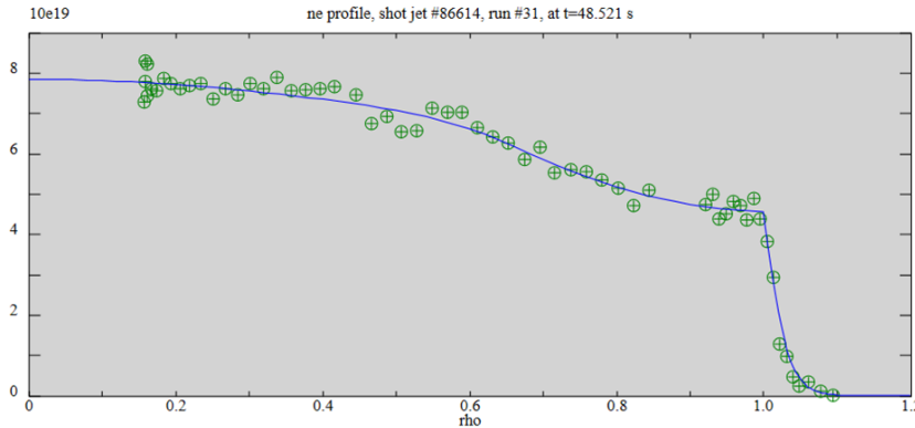
Figure 6: Fit of the electron density profile for a time slice of a JET shot (blue line), as a function of the normalised square root of the poloidal flux, obtained with a profile fitting tool developed for the IMAS Data Model. The fit was constrained from High Resolution Thomson Scattering (green crossed circles) measurements.
