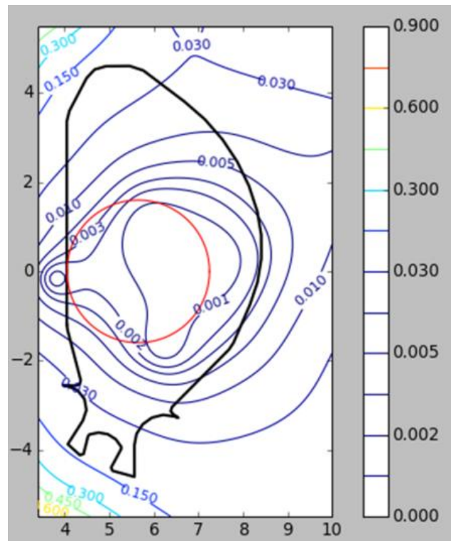
Figure 7: Magnetic field contours in ITER calculated for inboard start-up scenario
