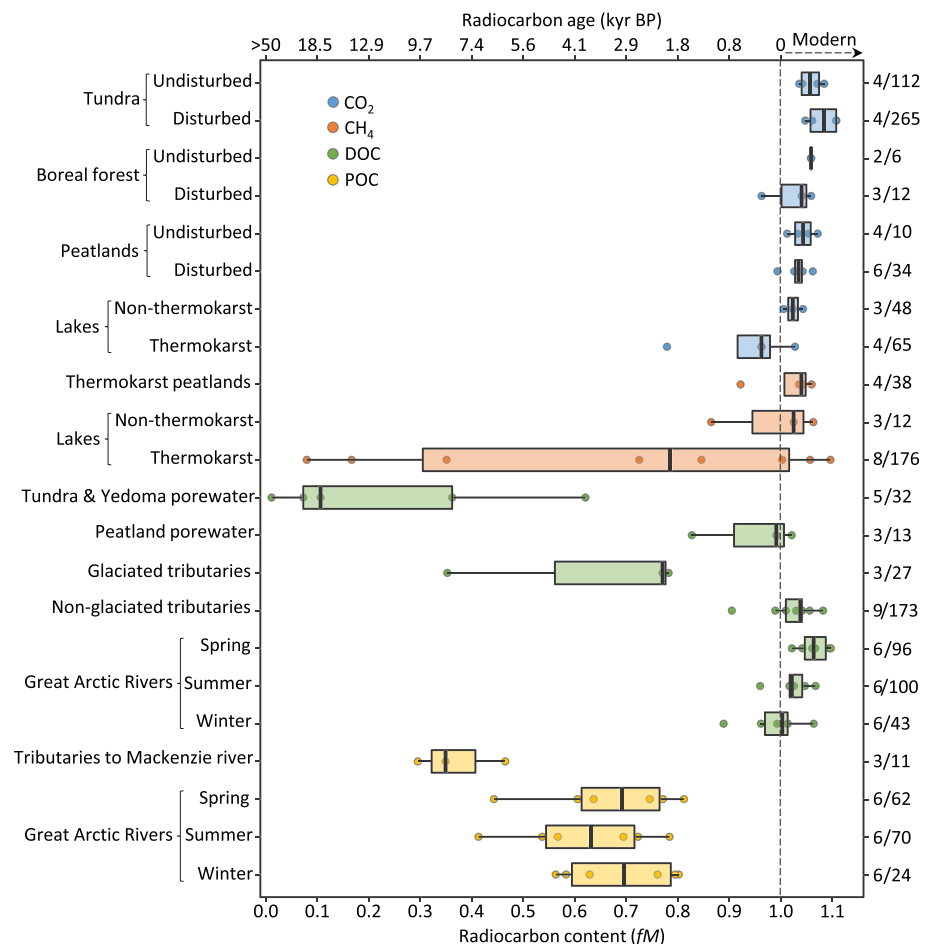
Figure 3. Summary of radiocarbon content of \text{CO}_2 , \text{CH}_4 , DOC, and POC measured in the northern permafrost region. Data for \text{CO}_2 and \text{CH}_4 refers to flux measurements released to the atmosphere and excludes belowground and soil incubation measurements, whereas data for DOC and POC includes both flux and belowground measurements to highlight the soil-stream-river continuum. Disturbance includes field manipulations (warming/wetting/drying), natural or fire-induced deepening of the active layer, and thermokarst processes. Each point represents the median of ^{14}\text{C} measurements from each study site (Table S1 shows the classification of sites and associated number of measurements). The boxes show the first and third quartiles, the solid vertical line is the median of medians, and the whiskers extend 1.5 times the interquartile range. On the right, the first value indicates the number of study sites and the second value indicates the total number of ^{14}\text{C} measurements.
