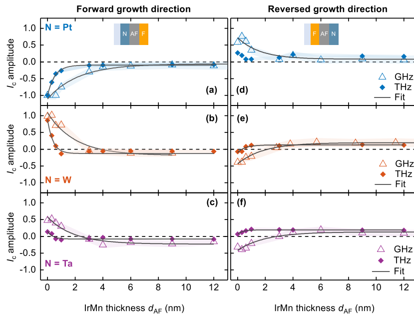
FIG. 2. | Impact of IrMn thickness on GHz and THz charge current. (a) Amplitude of charge currents I_c as a function of the IrMn thickness in Ni|IrMn|NiFe for N = Pt, (b) N = W and (c) N = Ta layer at both frequency ranges (GHz: open triangles, THz: closed diamonds). The data are normalized to I_c amplitudes obtained from Pt|IrMn( d_{AF} = 0 )|NiFe in GHz and THz sets, resulting in the effective spin-to-charge current conversion (S2C) efficiency relative to Pt|NiFe. (d–f) Same as (a–c), but for reversely grown NiFe|IrMn|N stacks. The data is normalized to account for thickness-dependent photonic and electronic effects unrelated to S2C. Errors are comparable to symbol sizes. The thick solid lines are guides to the eye. Fits (dark-gray thin solid lines) are offset mono-exponentials, giving the characteristic propagation lengths in IrMn. The fit values are summarized in Tab. 1 and Tab. S1.
