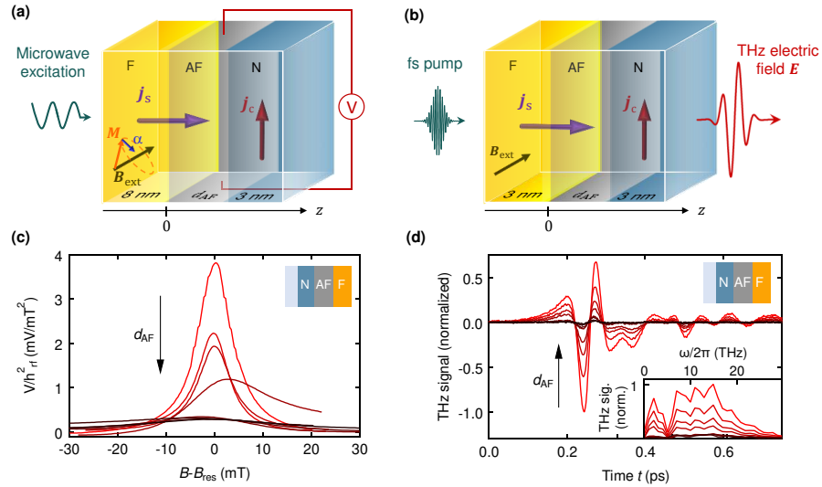
FIG. 1. | Measuring inverse spin Hall effect at GHz and THz frequencies. (a) Schematic of the GHz experiment. A microwave magnetic field (amplitude h_{rf} \sim 0.05 mT, frequency 9.6 GHz) triggers the precession of magnetization in a magnetic layer (F = NiFe, thickness of 8 nm) and, due to spin pumping, launches a periodic spin current j_s through the antiferromagnetic layer IrMn (AF, thickness d_{AF} ) into a heavy metal layer (N, 3 nm) where it is converted into a detectable DC charge current j_c via the inverse spin Hall effect. We note that the generated electric field is constant over the entire thickness of the thin-film stack. (b) The analogous experiment performed at THz frequencies. A femtosecond optical pulse triggers an ultrafast j_s between the magnetic (F, 3 nm) and the AF layer. The converted j_c serves as a source of an emitted THz pulse. (c, d) Typical raw experimental data, illustrated here by N = Pt: normalized voltage V/h_{rf} in the GHz (c) and the electro-optical signal in the THz (d) experiments for different d_{AF} (black arrows indicate increase of d_{AF} ). All waveforms in (d) were normalized by the amplitude corresponding to d_{AF} = 0 . Inset: amplitude spectrum of the corresponding THz temporal waveforms.
