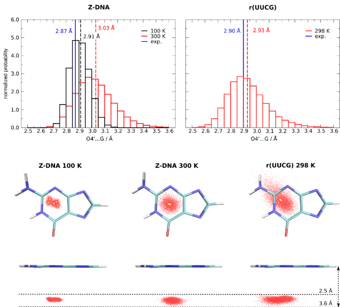
Figure 7. Histograms of O4'...G ( |\rho-\pi ) distances and top-down/side views on the O4'...G nucleobase from AFF MD simulations of Z-DNA and r(UUCG) tetraloop models. In the histograms the time-averaged O4'...G distances are marked by vertical dashed lines (black/100 K, red/300 K) while experimental values for Z-DNA (for 3P4J C 3 pG 4 and C 9 pG 10 steps) and r(UUCG) (2KOC, average from 20 models) are marked by blue solid lines. Projection points of the O4' atom on the G nucleobase are displayed as red points and averages for each combination of one CpG dinucleotide (for Z-DNA either 3-4 or 9-10) with one MD simulation are marked as yellow dots. In the top-down/side views on the O4'...G nucleobase every 100 th snapshot is visualized.
