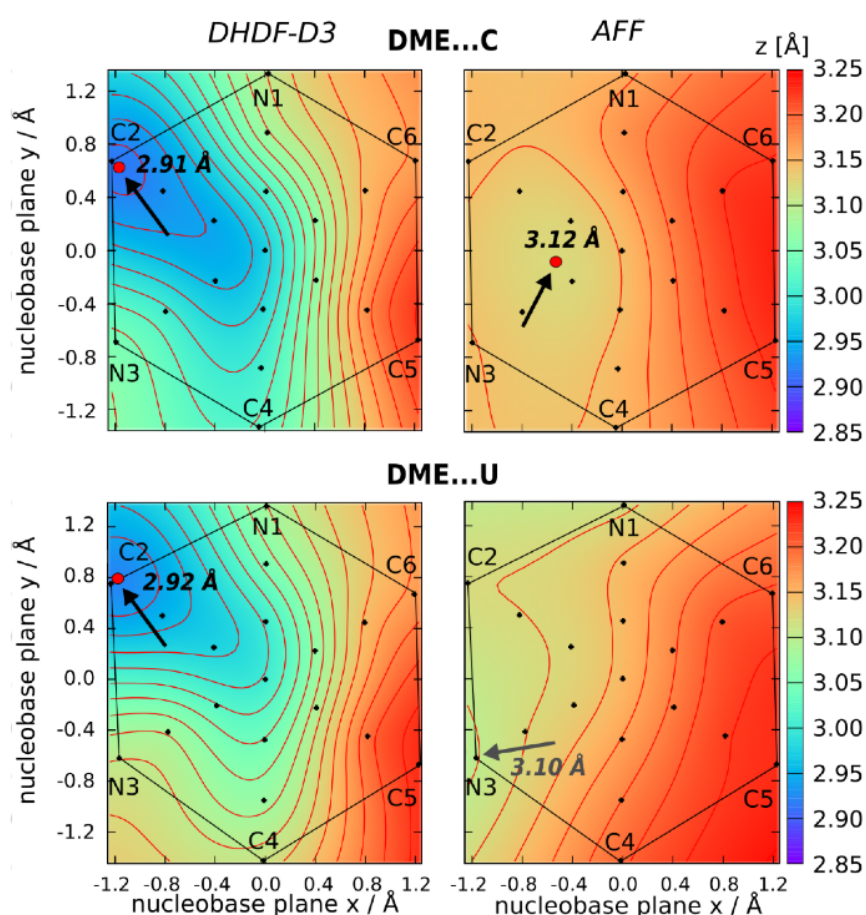
Figure 5. DME...C and DME...U minIEd surfaces for DHDF-D3 and AFF. Cytosine and uracil nucleobases lie in the xy plane. Color represents the 'z' coordinate of the O4' DME atom, the contours represent isoline stepping of 0.02 Å. The color scale is the same for all plots to ease visual comparison. Black arrows and distance values point to minima of the minIEd surfaces marked by red dots; small black dots mark points where the vertical scans were calculated (see also Figure S1). Note that for DME...U no AFF minIEd minimum is defined as it is outside the ring beyond the N3 atom. In this case, a grey arrow points to the N3 atom and the minIEd distance from vertical scan above the N3 atom is written in the graph. The AFF vs. DHDF-D3 difference range is 0.01 – 0.23 Å and 0.00 – 0.20 Å for C and U, respectively.
