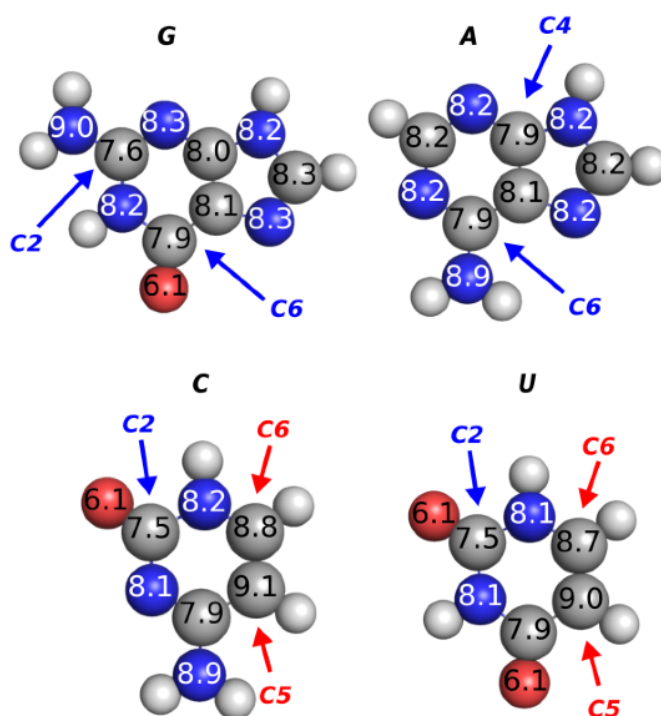
Figure 6. DFT-D4 based Atom-In-Molecule (AIM) polarizabilities \alpha(0) representing the volume of atoms in atomic units of cubic bohr ( a_0^3 ) for the four nucleobases guanine (G), adenine (A), cytosine (C) and uracil (U). The carbons discussed in the text are marked by blue (smaller carbon atoms) or red (larger carbon atoms) arrows.
