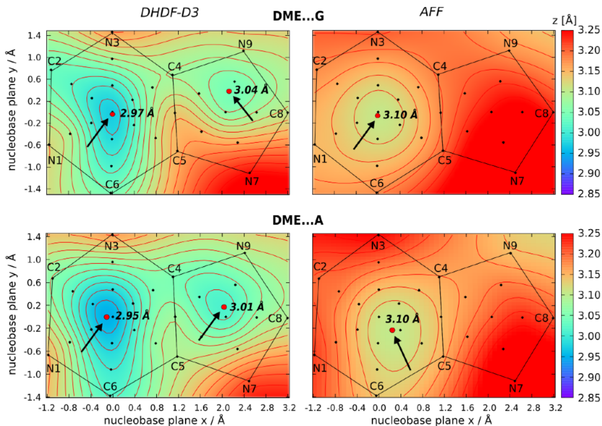
Figure 4. DME...G and DME...A minEd surfaces for DHDF-D3 and AFF. Guanine and adenine nucleobases lie in the xy plane. Color represents the ' z ' coordinate of the O4' DME atom, the contours represent isoline stepping of 0.02 Å. The color scale is the same for all plots to ease visual comparison. This causes a region of the AMBER surface around the N7 atom to be imprecisely represented as it slightly exceeds the scale. Black arrows and distance values point to minima of the minEd surfaces marked by red dots; small black dots mark nucleobase points where the vertical scans were calculated (see also Figure S1 ). The AFF vs. DHDF-D3 difference range is 0.03–0.18 Å and 0.05–0.19 Å for G and A, respectively. DHDF-D3 data for G are taken from Kruse et al. 17
