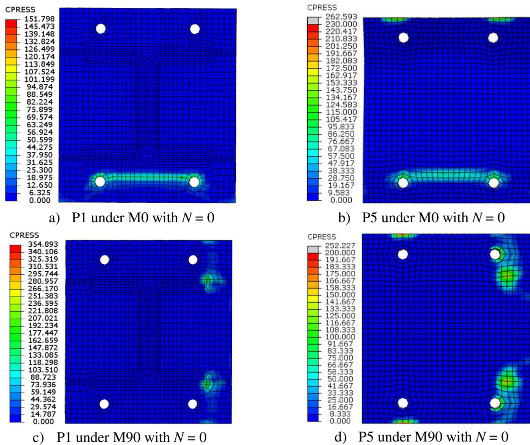
Fig. 16. Contact pressures of P1 and P5 at failure (in N/mm^2 )
