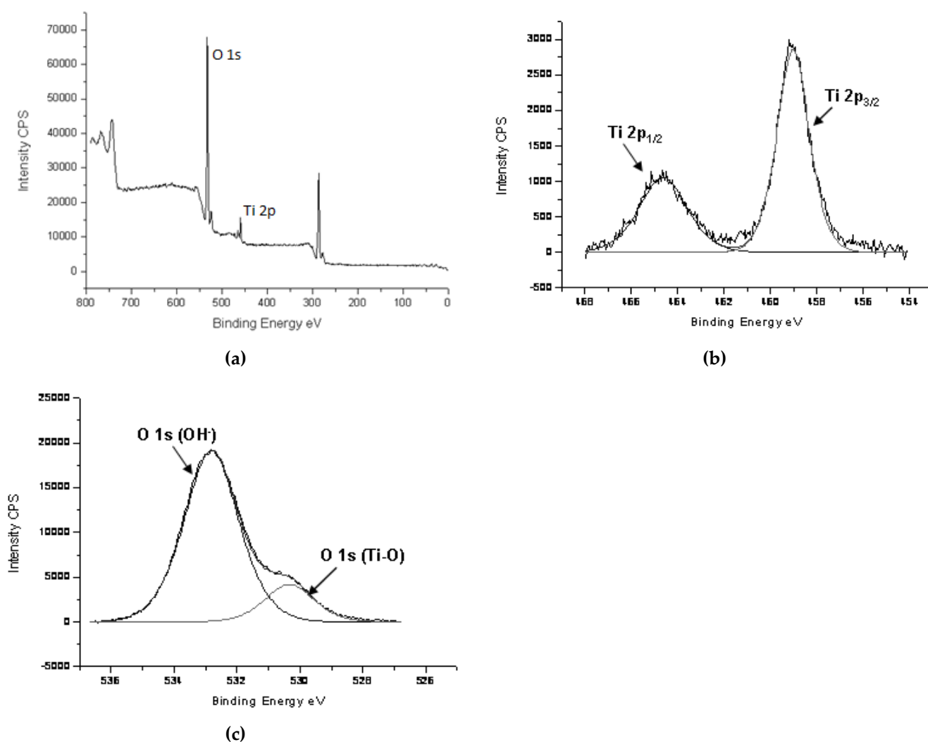
Figure 4. X-ray photoelectron spectra of the materials catalyst. (a) XPS survey Mg K \alpha photoelectron spectrum. (b) high-resolution XPS spectrum of the Ti 2p peaks. (c) High-resolution XPS spectrum of the O 1s peaks.
